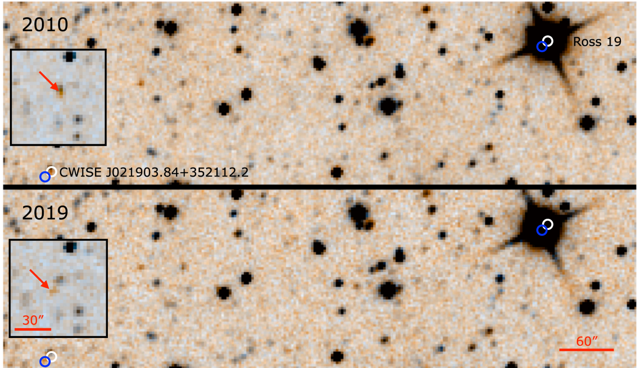
Figure 1. from Adam C. Schneider et al 2021 Astrophys. J. 921 doi:10.3847/1538-4357/ac1c75 https://dx.doi.org/10.3847/1538-4357/ac1c75 © 2021. The American Astronomical Society. All rights reserved.
