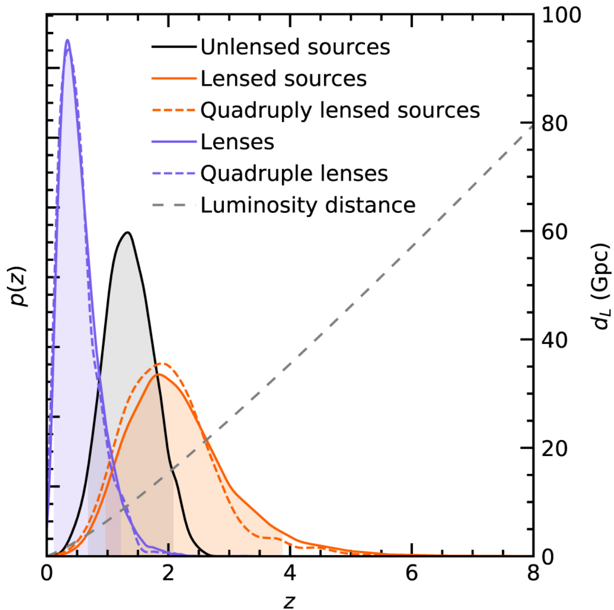
Figure 6. from A. Renske A. C. Wierda et al 2021 Astrophys. J. 921 doi:10.3847/1538-4357/ac1bb4 https://dx.doi.org/10.3847/1538-4357/ac1bb4 © 2021. The American Astronomical Society. All rights reserved.
