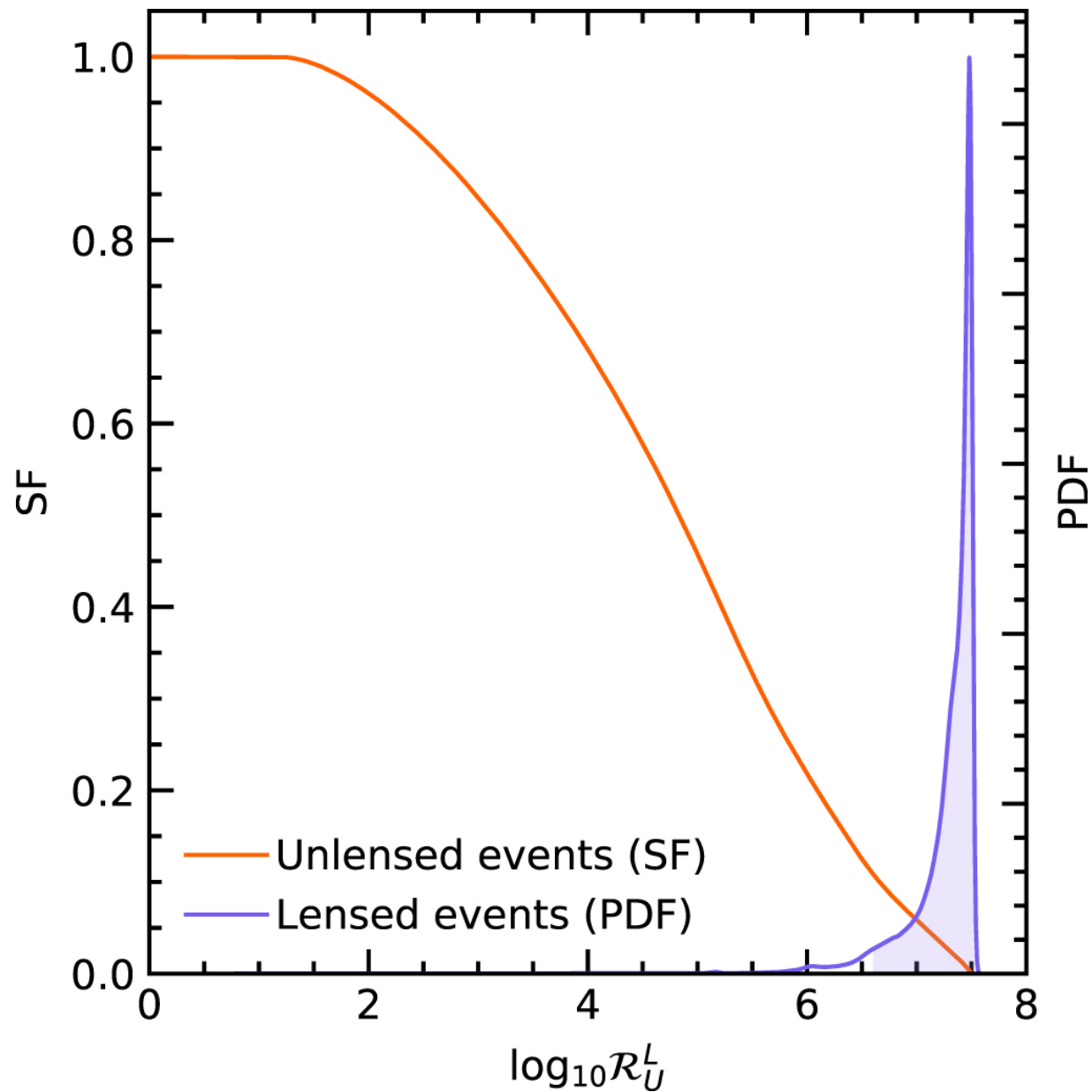
Figure 4. from A. Renske A. C. Wierda et al 2021 Astrophys. J. 921 doi:10.3847/1538-4357/ac1bb4 https://dx.doi.org/10.3847/1538-4357/ac1bb4 © 2021. The American Astronomical Society. All rights reserved.
