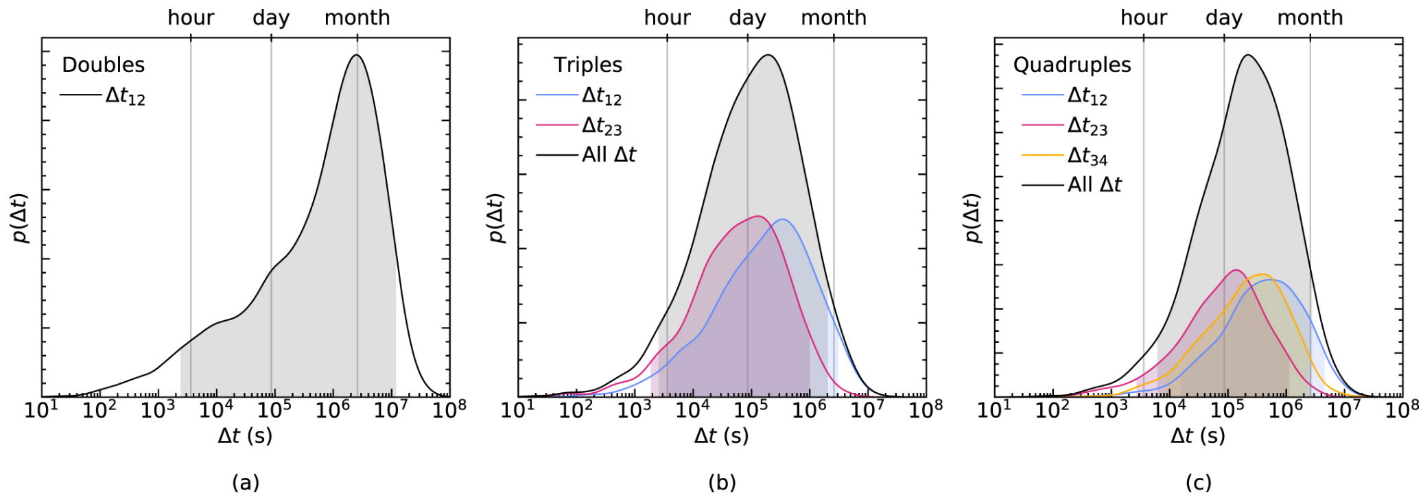
Figure 2. from A. Renske A. C. Wierda et al 2021 Astrophys. J. 921 doi:10.3847/1538-4357/ac1bb4 https://dx.doi.org/10.3847/1538-4357/ac1bb4 © 2021. The American Astronomical Society. All rights reserved.
