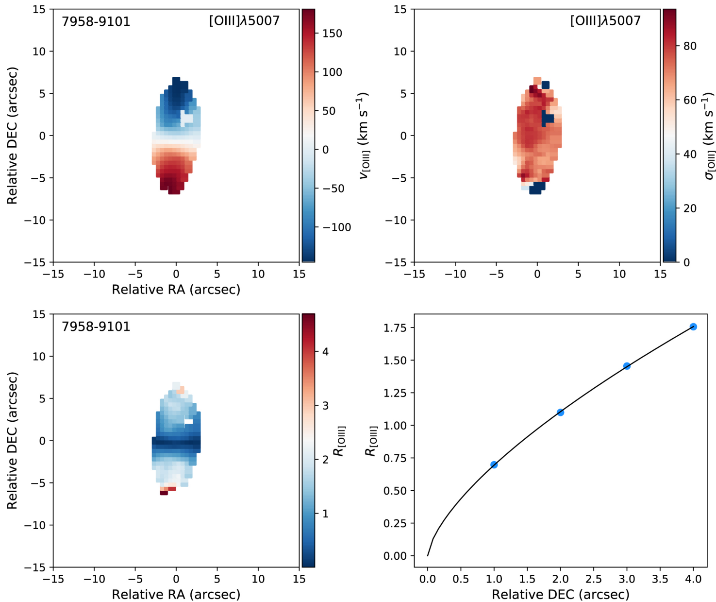
Figure 6. from Fabio Pacucci et al 2021 Astrophys. J. 920 doi:10.3847/1538-4357/ac1595 https://dx.doi.org/10.3847/1538-4357/ac1595 © 2021. The American Astronomical Society. All rights reserved.
