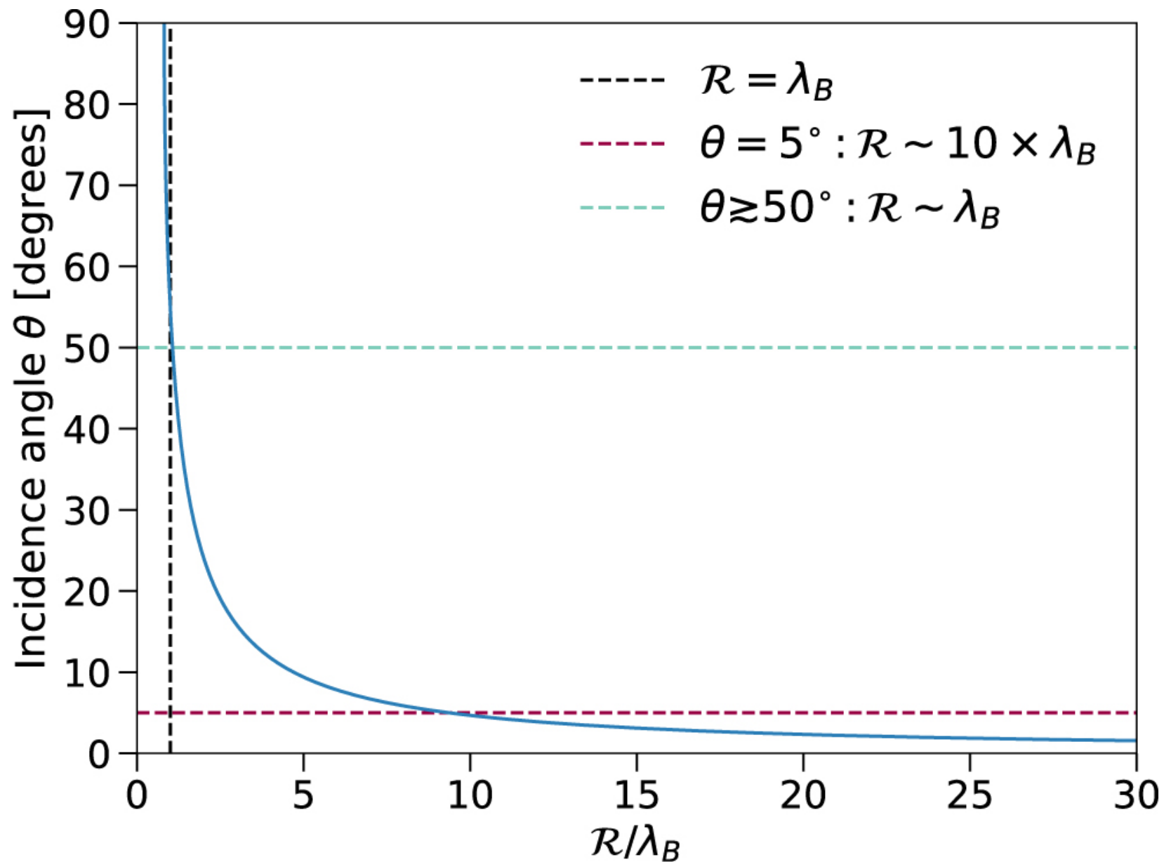
Figure 5. from Fabio Pacucci et al 2021 Astrophys. J. 920 doi:10.3847/1538-4357/ac1595 https://dx.doi.org/10.3847/1538-4357/ac1595 © 2021. The American Astronomical Society. All rights reserved.
