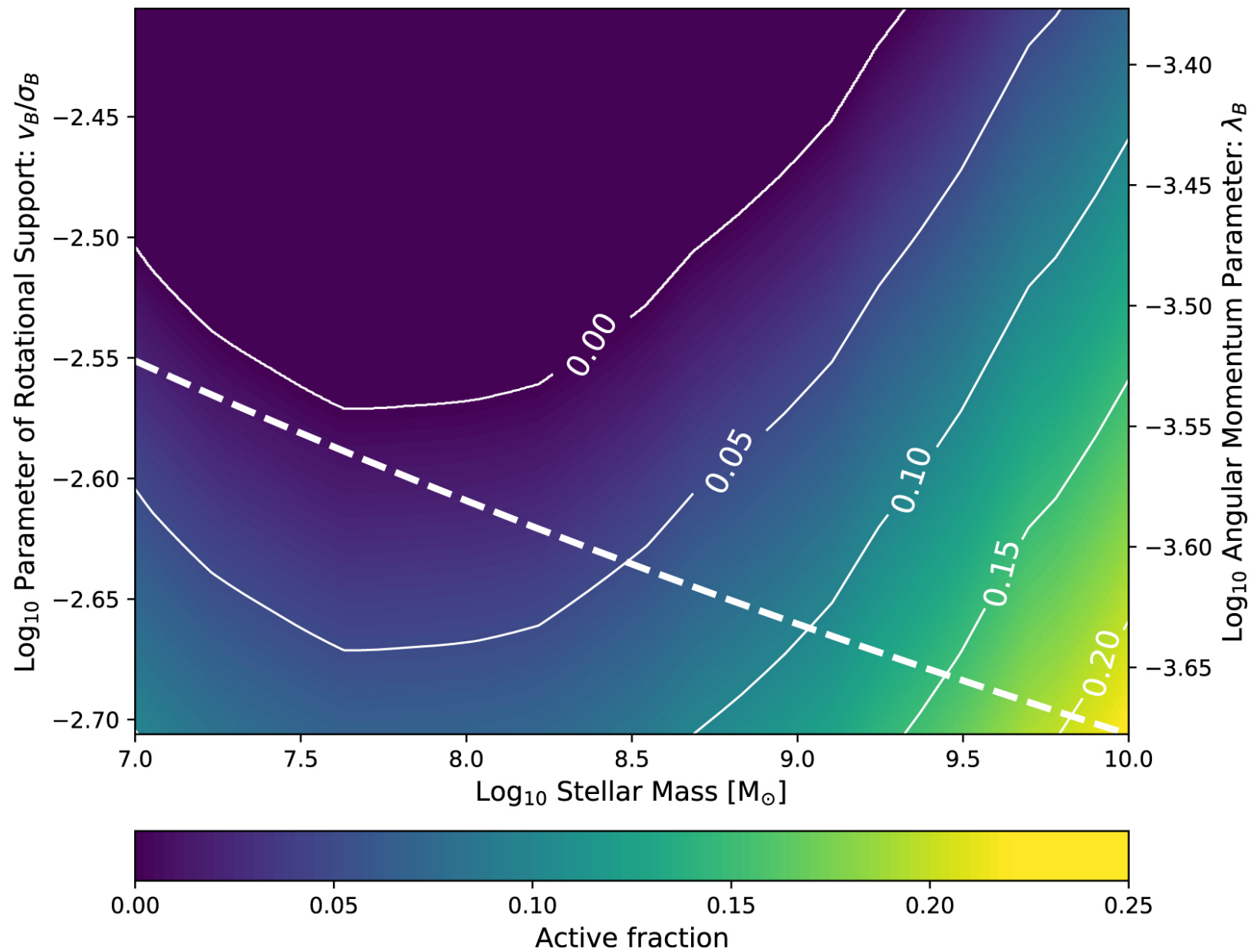
Figure 4. from Fabio Pacucci et al 2021 Astrophys. J. 920 doi:10.3847/1538-4357/ac1595 https://dx.doi.org/10.3847/1538-4357/ac1595 © 2021. The American Astronomical Society. All rights reserved.
