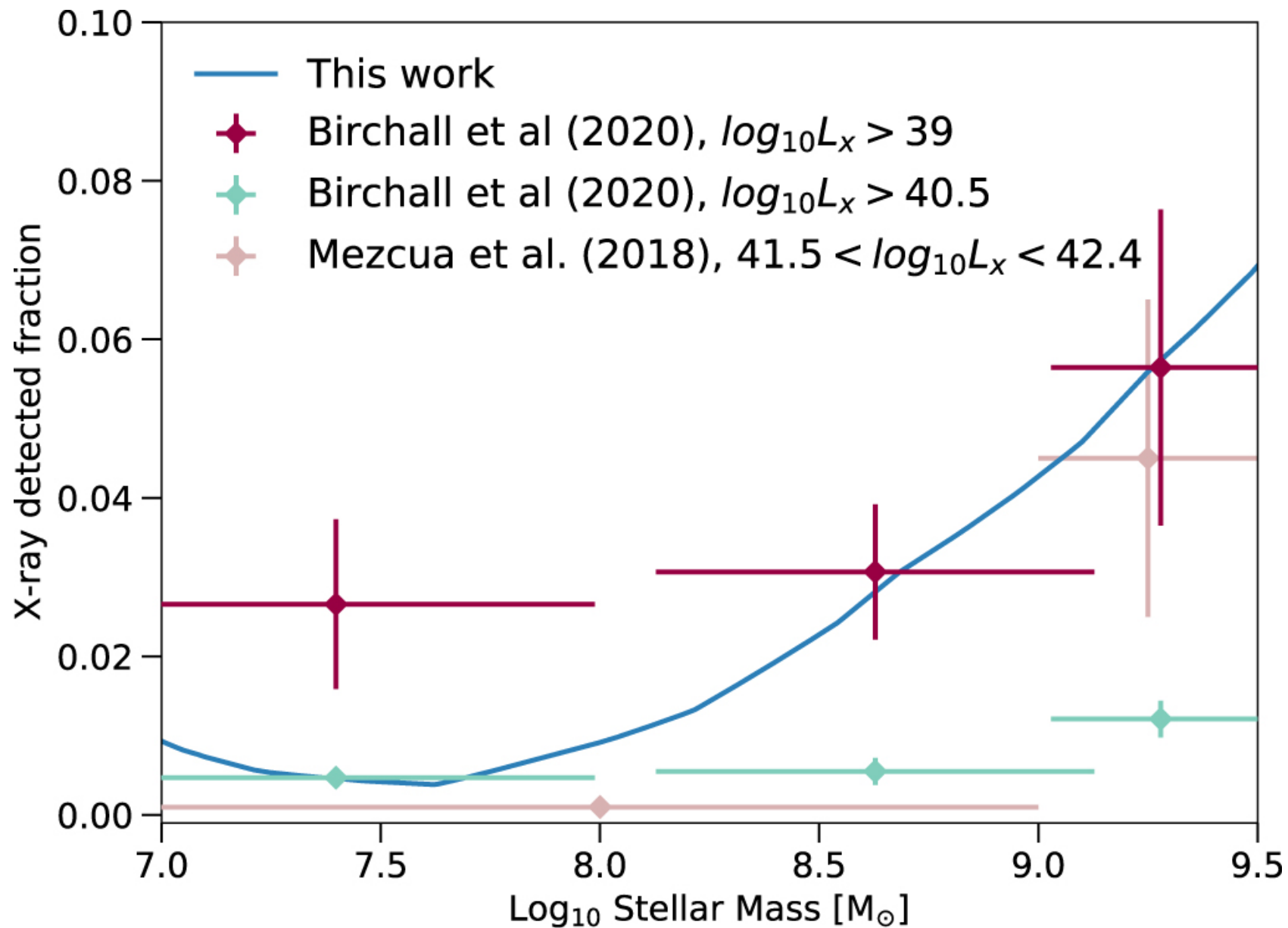
Figure 2. from Fabio Pacucci et al 2021 Astrophys. J. 920 doi:10.3847/1538-4357/ac1595 https://dx.doi.org/10.3847/1538-4357/ac1595 © 2021. The American Astronomical Society. All rights reserved.
