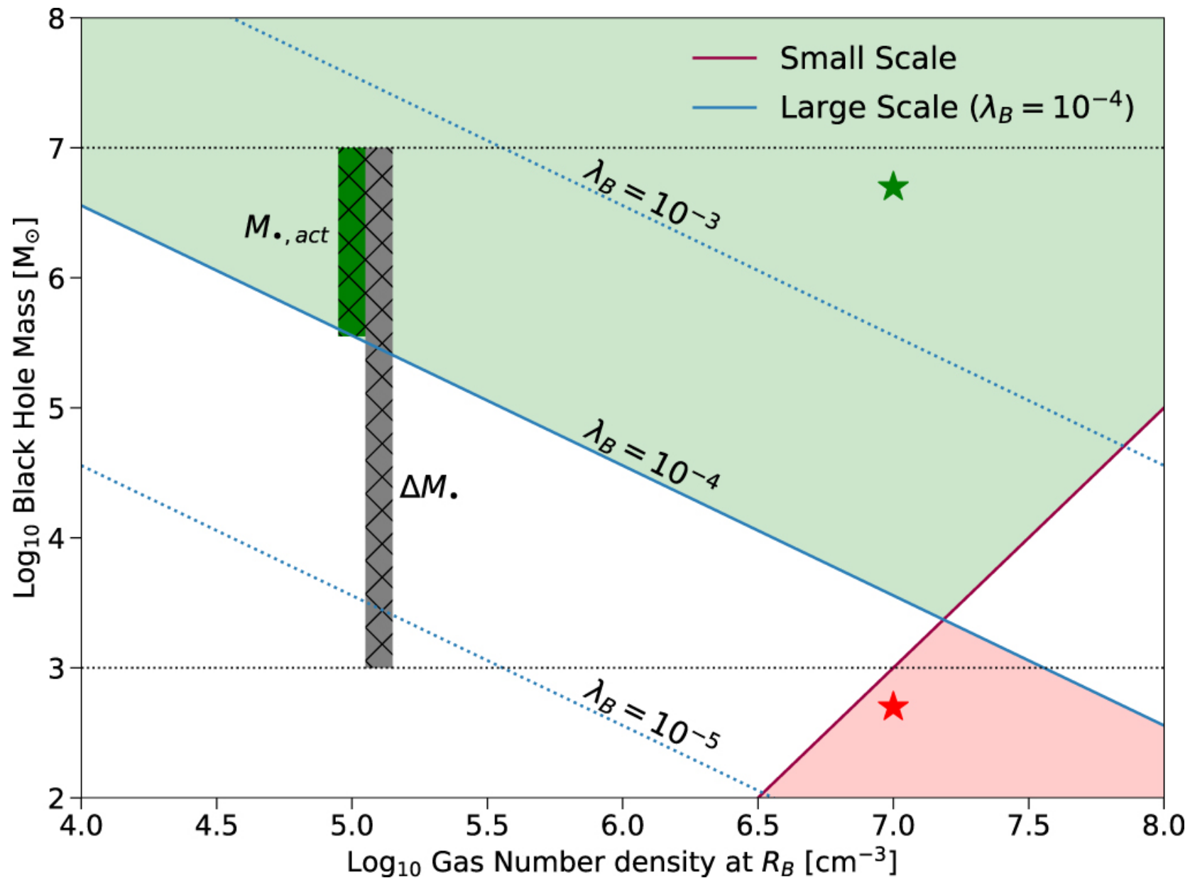
Figure 1. from Fabio Pacucci et al 2021 Astrophys. J. 920 doi:10.3847/1538-4357/ac1595 https://dx.doi.org/10.3847/1538-4357/ac1595 © 2021. The American Astronomical Society. All rights reserved.
