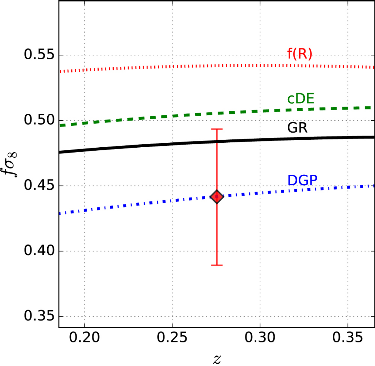
Figure 9. from C3 Cluster Clustering Cosmology I. New Constraints on the Cosmic Growth Rate at z \sim 0.3 from Redshift-space Clustering Anisotropies null 2021 APJ 920 13 doi:10.3847/1538-4357/ac0e8c https://dx.doi.org/10.3847/1538-4357/ac0e8c © 2021. The American Astronomical Society. All rights reserved.
