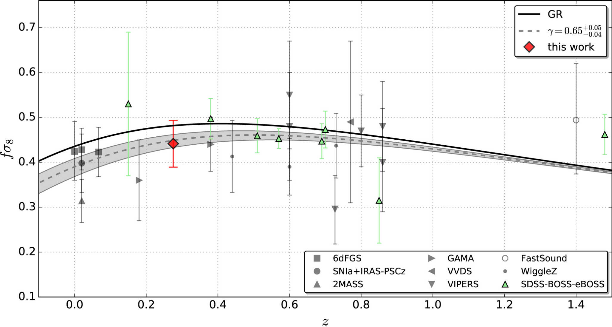
Figure 8. from C3 Cluster Clustering Cosmology I. New Constraints on the Cosmic Growth Rate at z \sim 0.3 from Redshift-space Clustering Anisotropies null 2021 APJ 920 13 doi:10.3847/1538-4357/ac0e8c https://dx.doi.org/10.3847/1538-4357/ac0e8c © 2021. The American Astronomical Society. All rights reserved.
