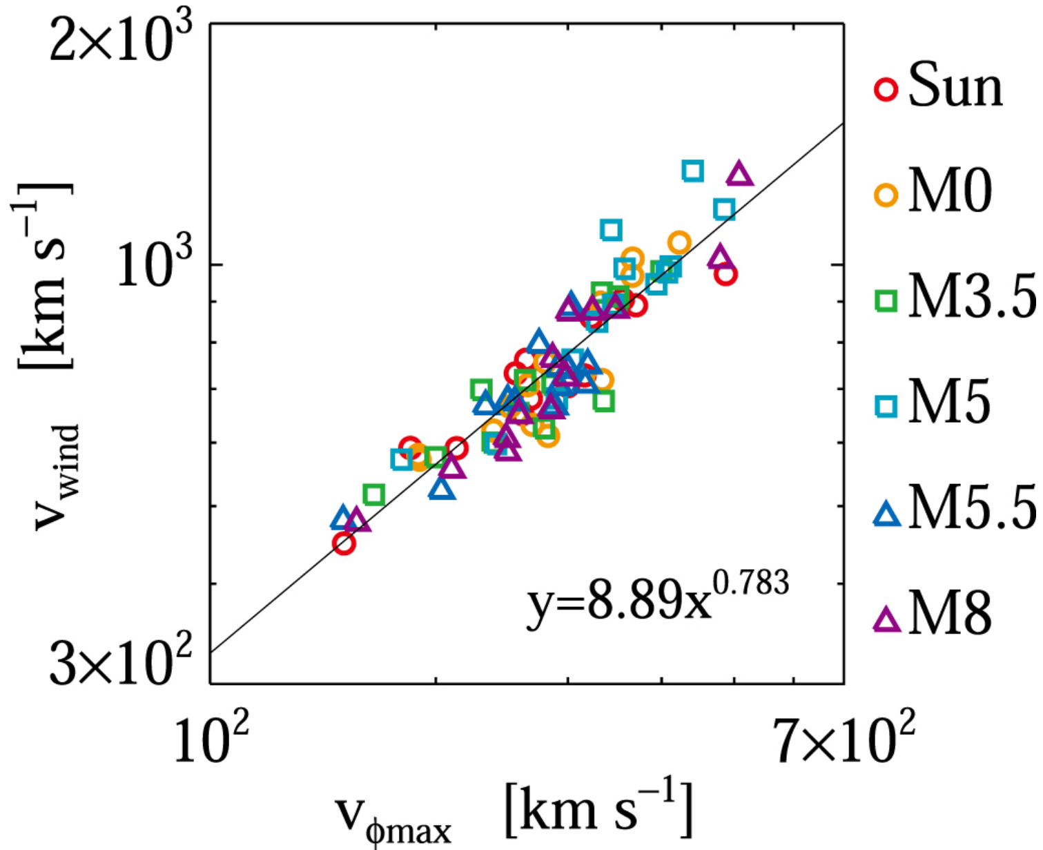
Figure 9. from An M Dwarf's Chromosphere, Corona, and Wind Connection via Nonlinear Alfvén Waves null 2021 APJ 919 29 doi:10.3847/1538-4357/ac0e34 https://dx.doi.org/10.3847/1538-4357/ac0e34 © 2021. The American Astronomical Society. All rights reserved.
