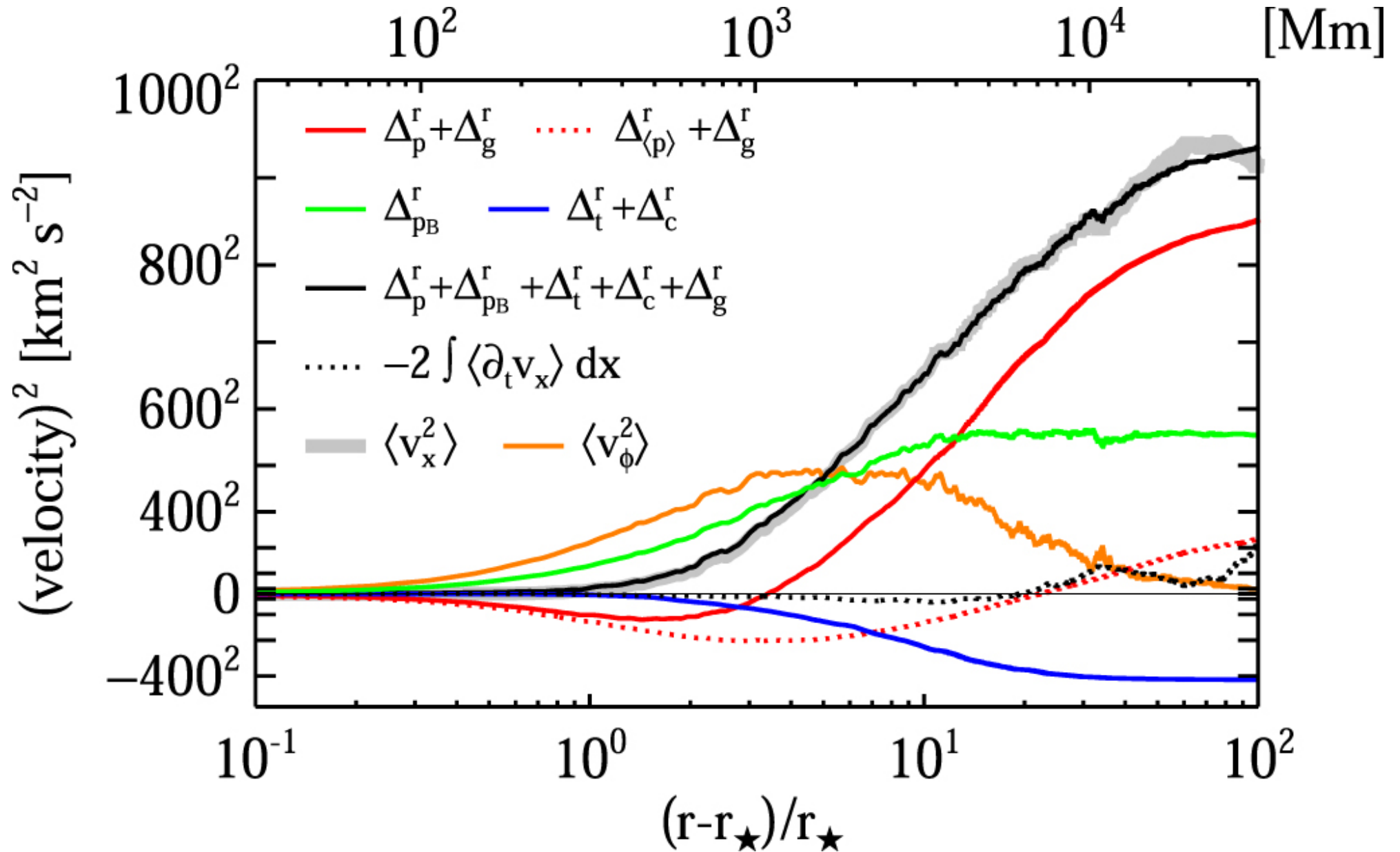
Figure 7. from An M Dwarf's Chromosphere, Corona, and Wind Connection via Nonlinear Alfvén Waves null 2021 APJ 919 29 doi:10.3847/1538-4357/ac0e34 https://dx.doi.org/10.3847/1538-4357/ac0e34 © 2021. The American Astronomical Society. All rights reserved.
