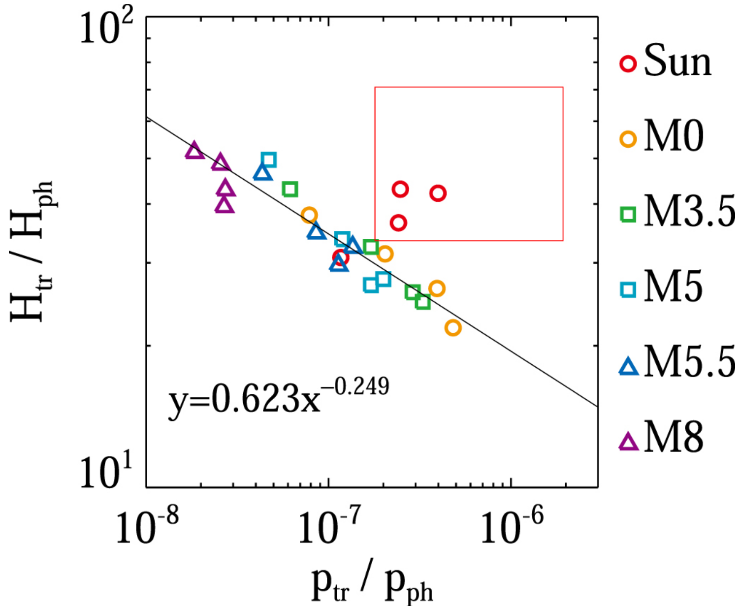
Figure 6. from An M Dwarf's Chromosphere, Corona, and Wind Connection via Nonlinear Alfvén Waves null 2021 APJ 919 29 doi:10.3847/1538-4357/ac0e34 https://dx.doi.org/10.3847/1538-4357/ac0e34 © 2021. The American Astronomical Society. All rights reserved.
