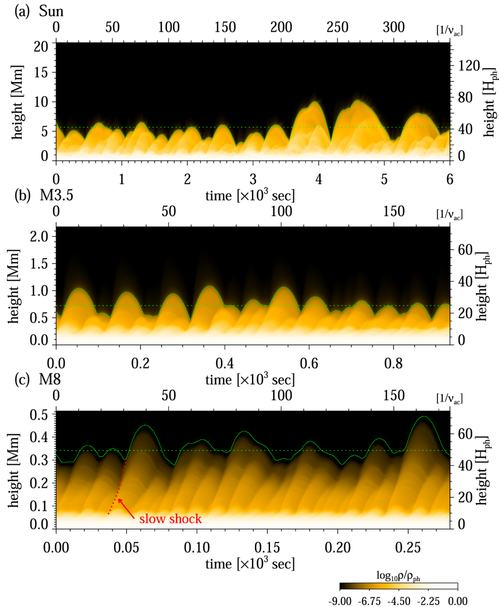
Figure 5. from An M Dwarf's Chromosphere, Corona, and Wind Connection via Nonlinear Alfvén Waves null 2021 APJ 919 29 doi:10.3847/1538-4357/ac0e34 https://dx.doi.org/10.3847/1538-4357/ac0e34
