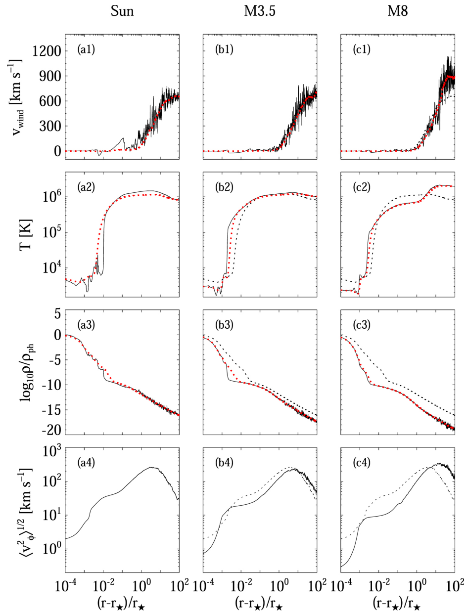
Figure 3. from An M Dwarf's Chromosphere, Corona, and Wind Connection via Nonlinear Alfvén Waves null 2021 APJ 919 29 doi:10.3847/1538-4357/ac0e34 https://dx.doi.org/10.3847/1538-4357/ac0e34 © 2021. The American Astronomical Society. All rights reserved.
