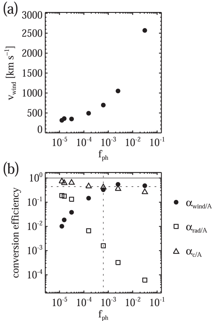
Figure 24. from An M Dwarf's Chromosphere, Corona, and Wind Connection via Nonlinear Alfvén Waves null 2021 APJ 919 29 doi:10.3847/1538-4357/ac0e34 https://dx.doi.org/10.3847/1538-4357/ac0e34 © 2021. The American Astronomical Society. All rights reserved.
