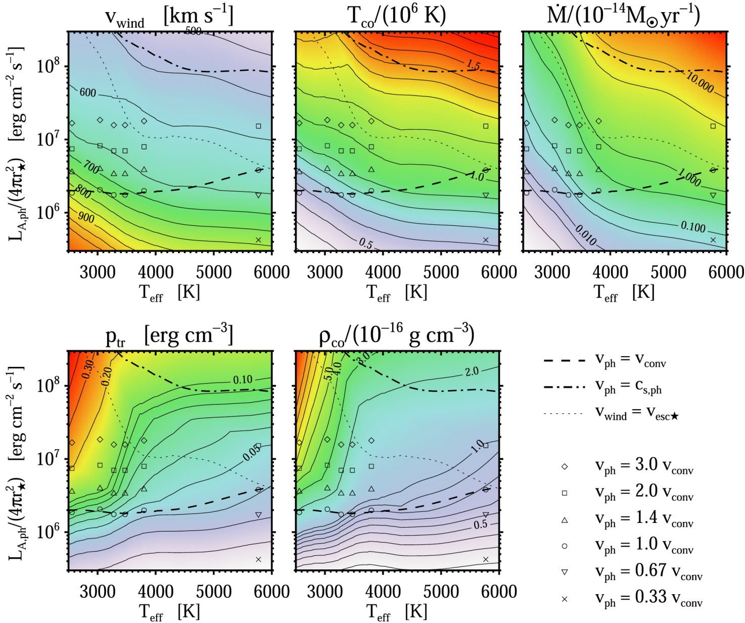
Figure 18. from An M Dwarf's Chromosphere, Corona, and Wind Connection via Nonlinear Alfvén Waves null 2021 APJ 919 29 doi:10.3847/1538-4357/ac0e34 https://dx.doi.org/10.3847/1538-4357/ac0e34
