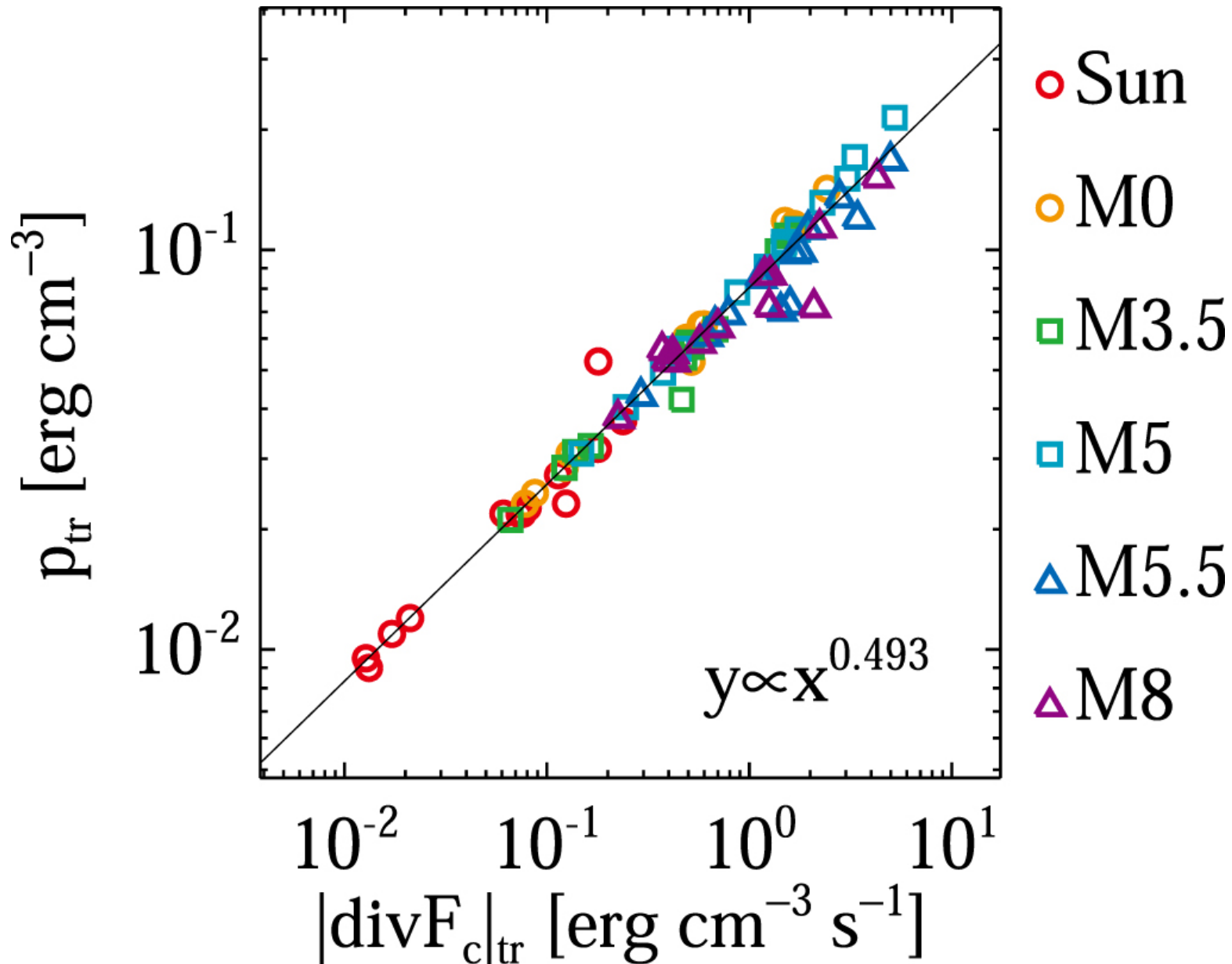
Figure 17. from An M Dwarf's Chromosphere, Corona, and Wind Connection via Nonlinear Alfvén Waves null 2021 APJ 919 29 doi:10.3847/1538-4357/ac0e34 https://dx.doi.org/10.3847/1538-4357/ac0e34 © 2021. The American Astronomical Society. All rights reserved.
