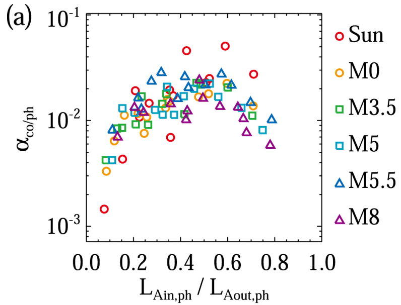
Figure 16. from An M Dwarf's Chromosphere, Corona, and Wind Connection via Nonlinear Alfvén Waves null 2021 APJ 919 29 doi:10.3847/1538-4357/ac0e34 https://dx.doi.org/10.3847/1538-4357/ac0e34 © 2021. The American Astronomical Society. All rights reserved.
