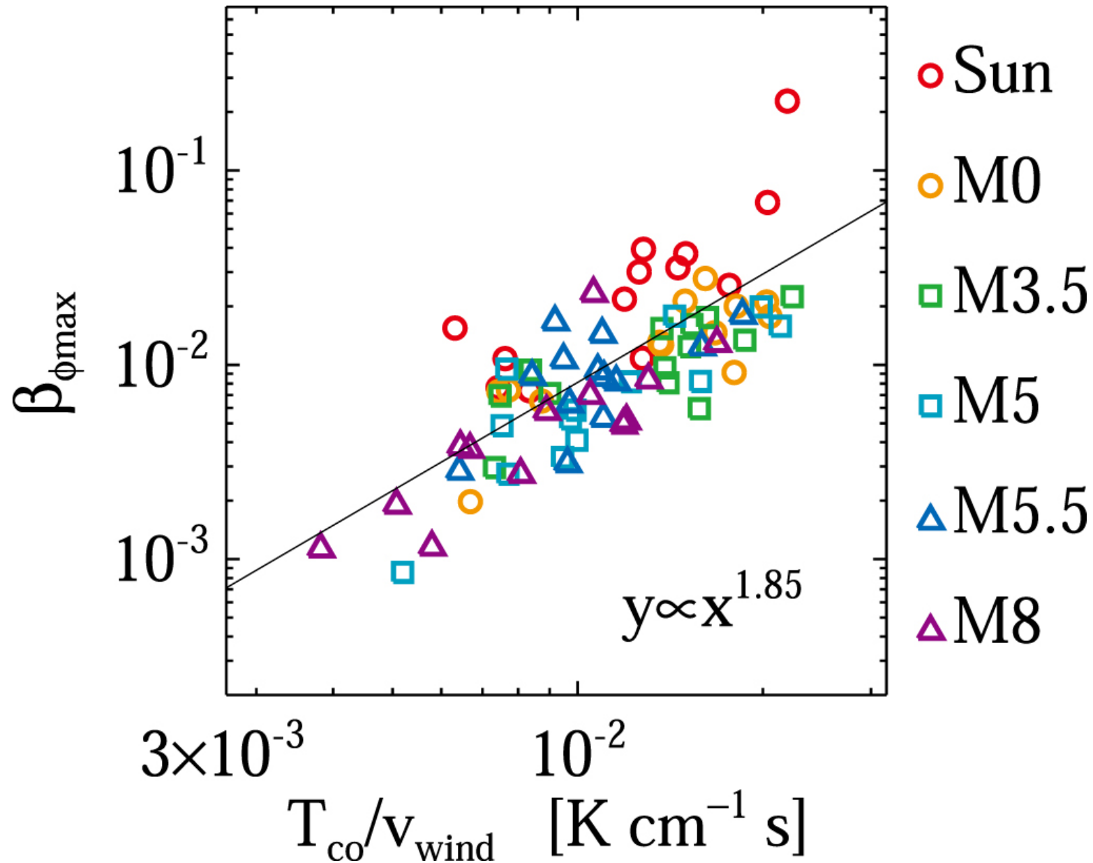
Figure 15. from An M Dwarf's Chromosphere, Corona, and Wind Connection via Nonlinear Alfvén Waves null 2021 APJ 919 29 doi:10.3847/1538-4357/ac0e34 https://dx.doi.org/10.3847/1538-4357/ac0e34 © 2021. The American Astronomical Society. All rights reserved.
