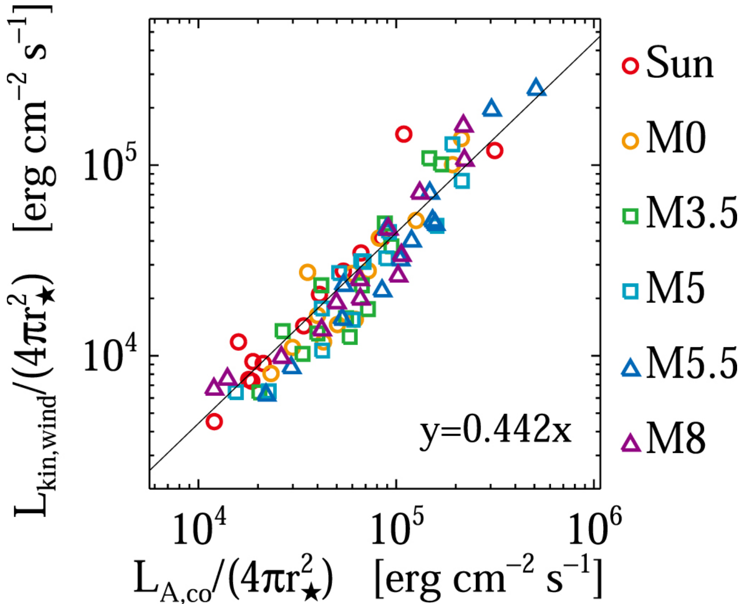
Figure 14. from An M Dwarf's Chromosphere, Corona, and Wind Connection via Nonlinear Alfvén Waves null 2021 APJ 919 29 doi:10.3847/1538-4357/ac0e34 https://dx.doi.org/10.3847/1538-4357/ac0e34 © 2021. The American Astronomical Society. All rights reserved.
