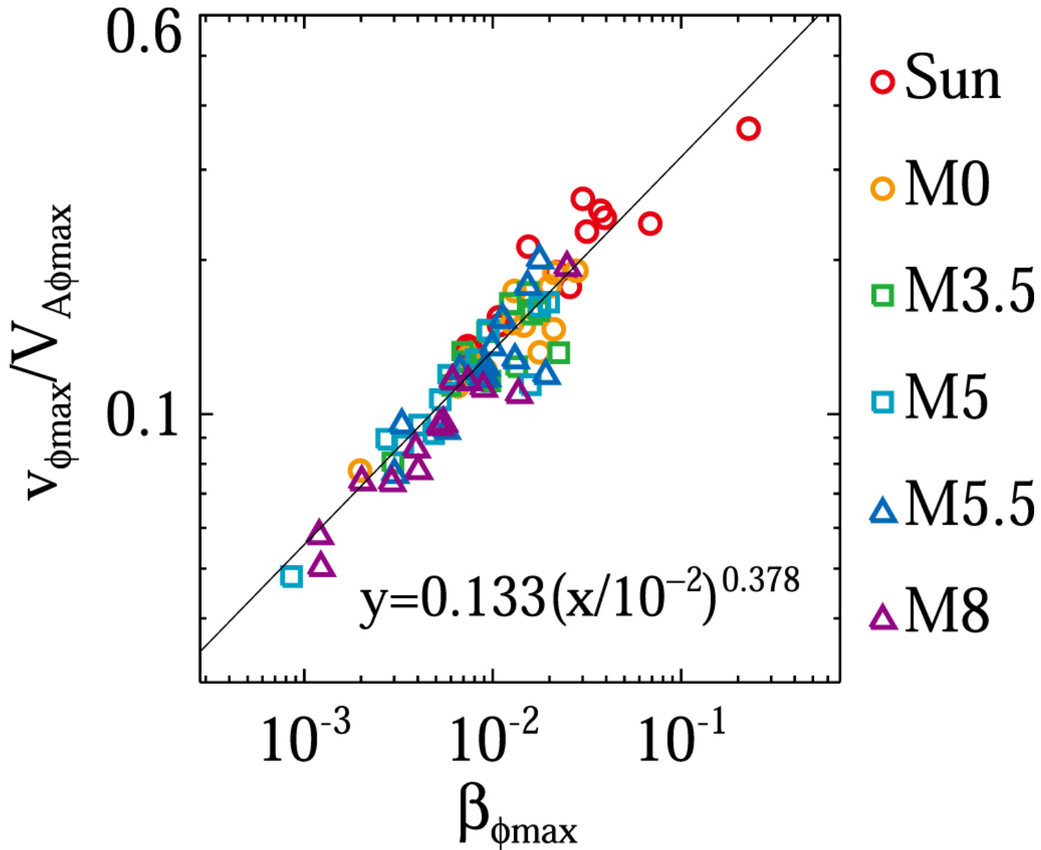
Figure 13. from An M Dwarf's Chromosphere, Corona, and Wind Connection via Nonlinear Alfvén Waves null 2021 APJ 919 29 doi:10.3847/1538-4357/ac0e34 https://dx.doi.org/10.3847/1538-4357/ac0e34 © 2021. The American Astronomical Society. All rights reserved.
