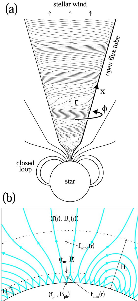
Figure 1. from An M Dwarf's Chromosphere, Corona, and Wind Connection via Nonlinear Alfvén Waves null 2021 APJ 919 29 doi:10.3847/1538-4357/ac0e34 https://dx.doi.org/10.3847/1538-4357/ac0e34 © 2021. The American Astronomical Society. All rights reserved.
