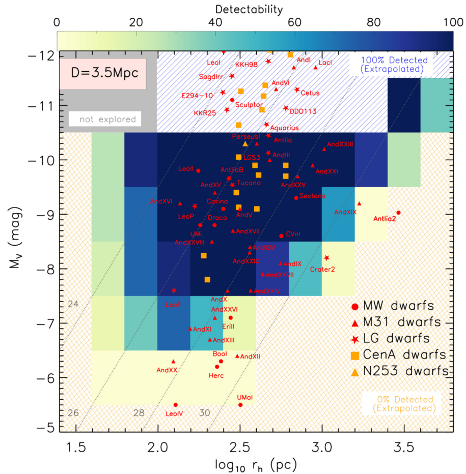
Figure 8. from Resolved Dwarf Galaxy Searches within 5 Mpc with the Vera Rubin Observatory and Subaru Hyper Suprime-Cam null 2021 APJ 918 88 doi:10.3847/1538-4357/ac0db8 https://dx.doi.org/10.3847/1538-4357/ac0db8 © 2021. The American Astronomical Society. All rights reserved.
