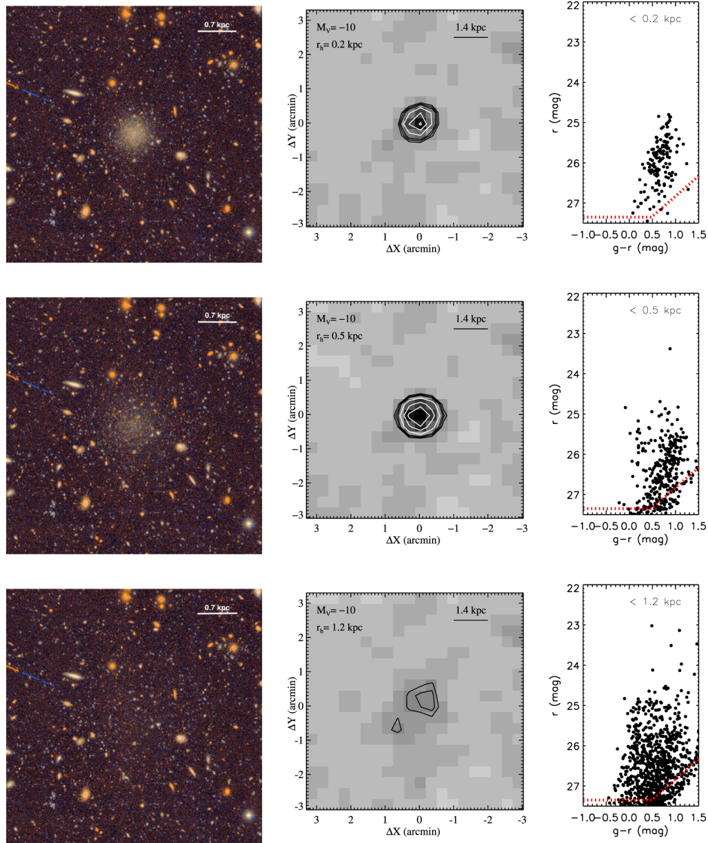
Figure 6. from Resolved Dwarf Galaxy Searches within 5 Mpc with the Vera Rubin Observatory and Subaru Hyper Suprime-Cam null 2021 APJ 918 88 doi:10.3847/1538-4357/ac0db8 https://dx.doi.org/10.3847/1538-4357/ac0db8 © 2021. The American Astronomical Society. All rights reserved.
