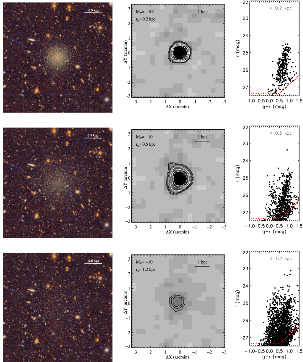
Figure 5. from Resolved Dwarf Galaxy Searches within 5 Mpc with the Vera Rubin Observatory and Subaru Hyper Suprime-Cam null 2021 APJ 918 88 doi:10.3847/1538-4357/ac0db8 https://dx.doi.org/10.3847/1538-4357/ac0db8 © 2021. The American Astronomical Society. All rights reserved.
