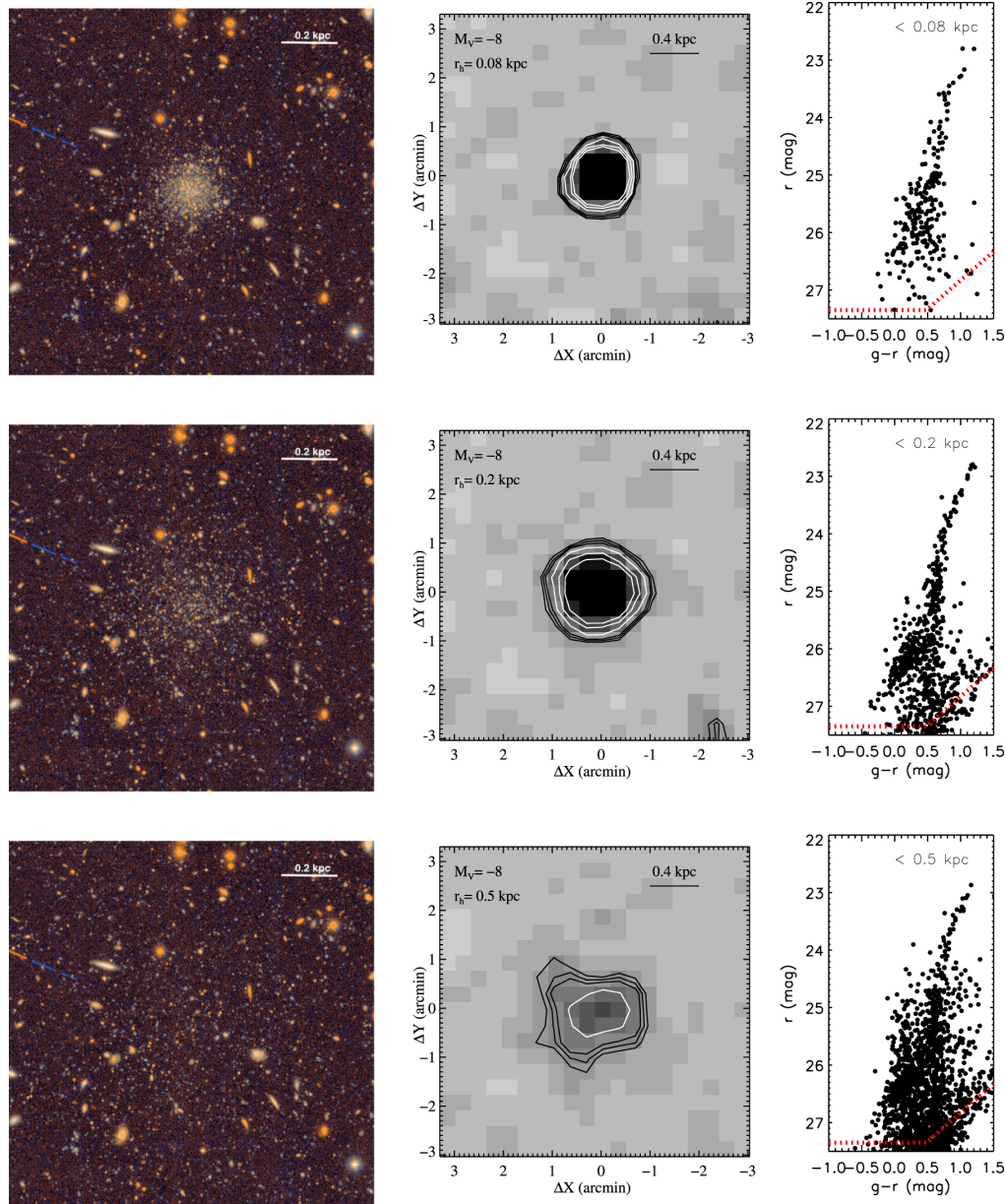
Figure 4. from Resolved Dwarf Galaxy Searches within 5 Mpc with the Vera Rubin Observatory and Subaru Hyper Suprime-Cam null 2021 APJ 918 88 doi:10.3847/1538-4357/ac0db8 https://dx.doi.org/10.3847/1538-4357/ac0db8 © 2021. The American Astronomical Society. All rights reserved.
