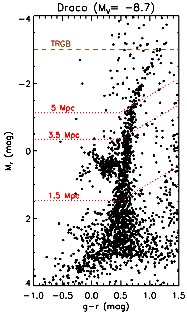
Figure 2. from Resolved Dwarf Galaxy Searches within 5 Mpc with the Vera Rubin Observatory and Subaru Hyper Suprime-Cam null 2021 APJ 918 88 doi:10.3847/1538-4357/ac0db8 https://dx.doi.org/10.3847/1538-4357/ac0db8 © 2021. The American Astronomical Society. All rights reserved.
