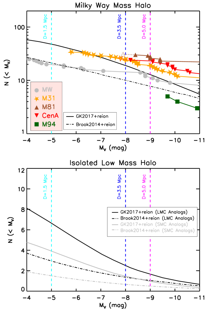
Figure 11. from Resolved Dwarf Galaxy Searches within 5 Mpc with the Vera Rubin Observatory and Subaru Hyper Suprime-Cam null 2021 APJ 918 88 doi:10.3847/1538-4357/ac0db8 https://dx.doi.org/10.3847/1538-4357/ac0db8 © 2021. The American Astronomical Society. All rights reserved.
