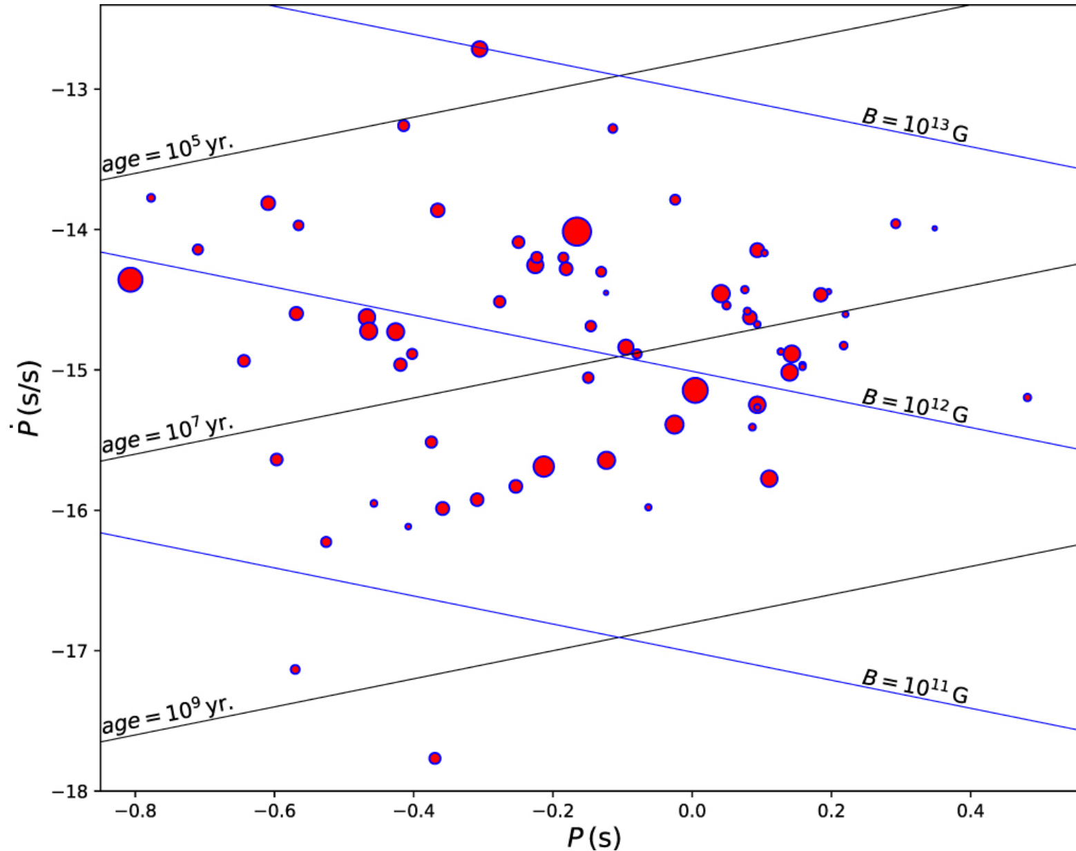
Figure 8. from A Systematic Study of the Frequency Evolution Behavior of Pulsar Pulse Profiles null 2021 APJ 917 108 doi:10.3847/1538-4357/ac0b40 https://dx.doi.org/10.3847/1538-4357/ac0b40 © 2021. The American Astronomical Society. All rights reserved.
