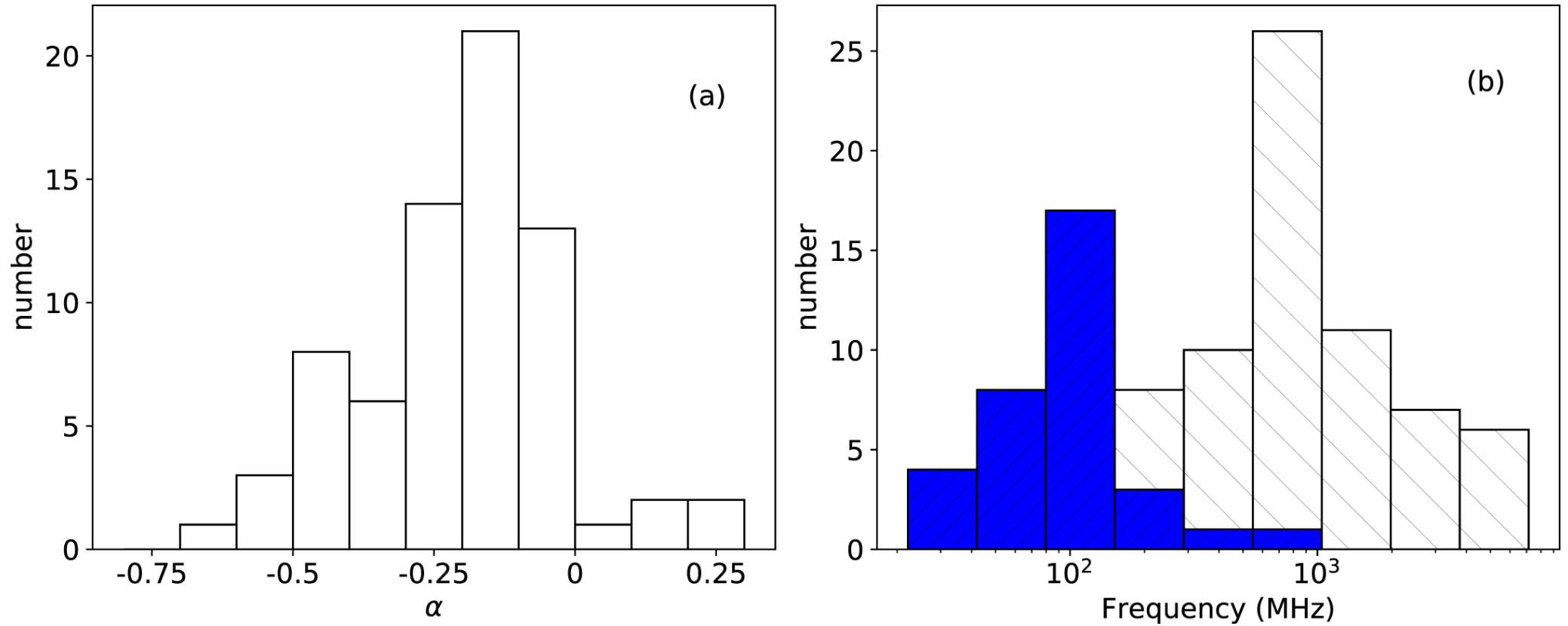
Figure 7. from A Systematic Study of the Frequency Evolution Behavior of Pulsar Pulse Profiles null 2021 APJ 917 108 doi:10.3847/1538-4357/ac0b40 https://dx.doi.org/10.3847/1538-4357/ac0b40 © 2021. The American Astronomical Society. All rights reserved.
