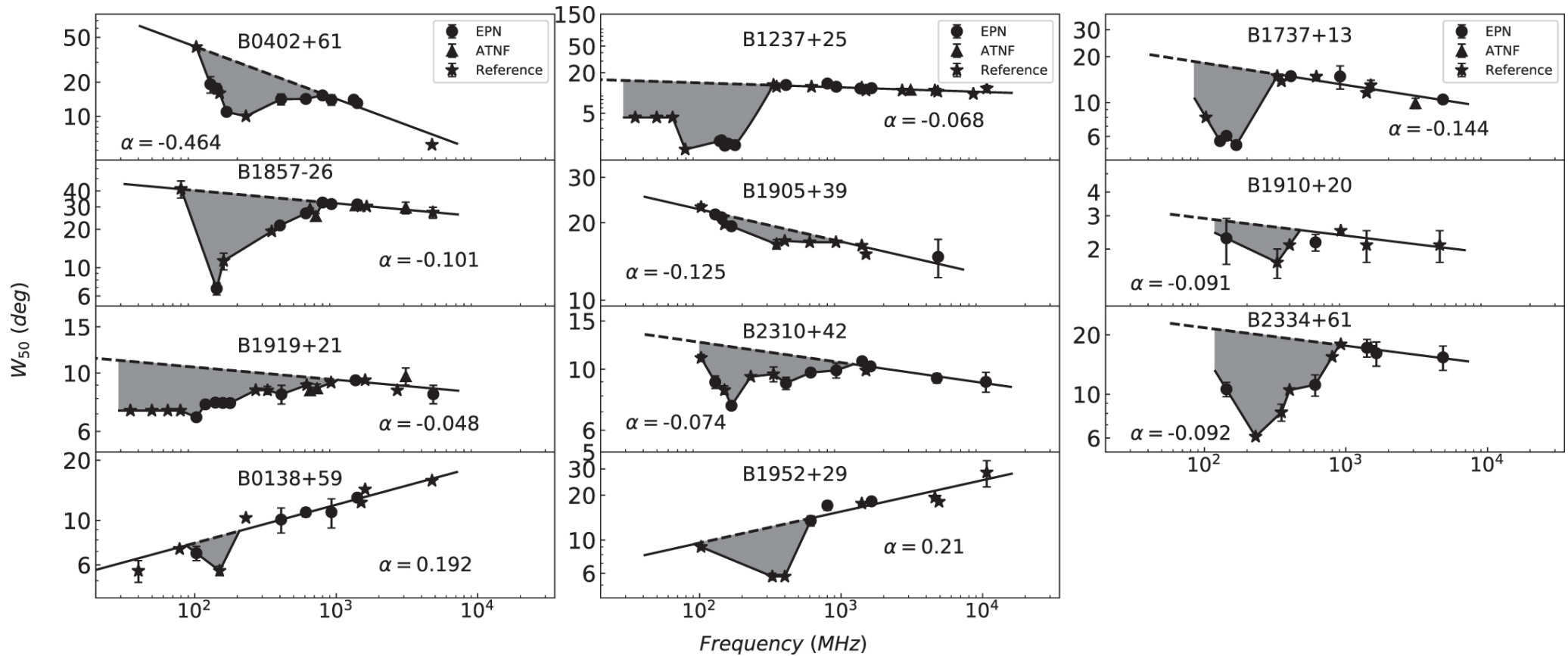
Figure 6. from A Systematic Study of the Frequency Evolution Behavior of Pulsar Pulse Profiles null 2021 APJ 917 108 doi:10.3847/1538-4357/ac0b40 https://dx.doi.org/10.3847/1538-4357/ac0b40 © 2021. The American Astronomical Society. All rights reserved.
