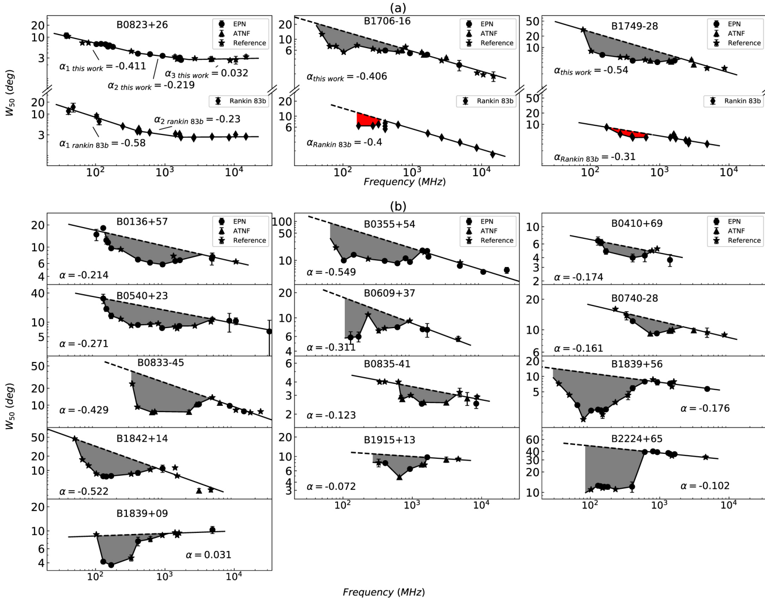
Figure 3. from A Systematic Study of the Frequency Evolution Behavior of Pulsar Pulse Profiles null 2021 APJ 917 108 doi:10.3847/1538-4357/ac0b40 https://dx.doi.org/10.3847/1538-4357/ac0b40 © 2021. The American Astronomical Society. All rights reserved.
