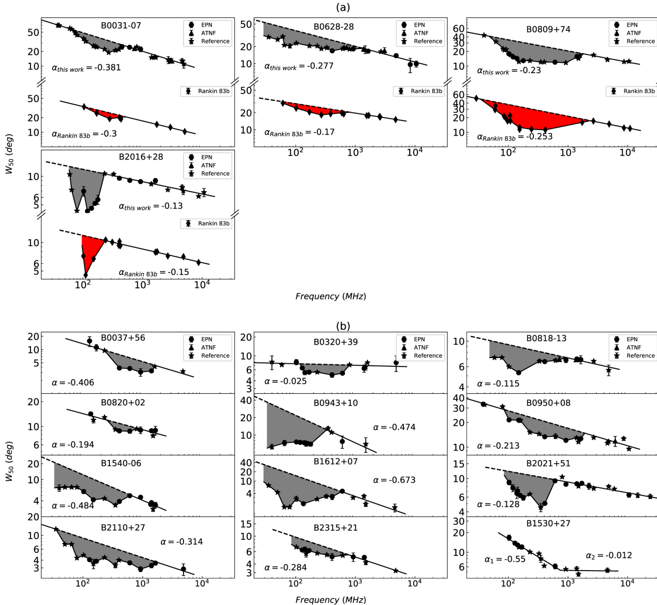
Figure 2. from A Systematic Study of the Frequency Evolution Behavior of Pulsar Pulse Profiles null 2021 APJ 917 108 doi:10.3847/1538-4357/ac0b40 https://dx.doi.org/10.3847/1538-4357/ac0b40 © 2021. The American Astronomical Society. All rights reserved.
