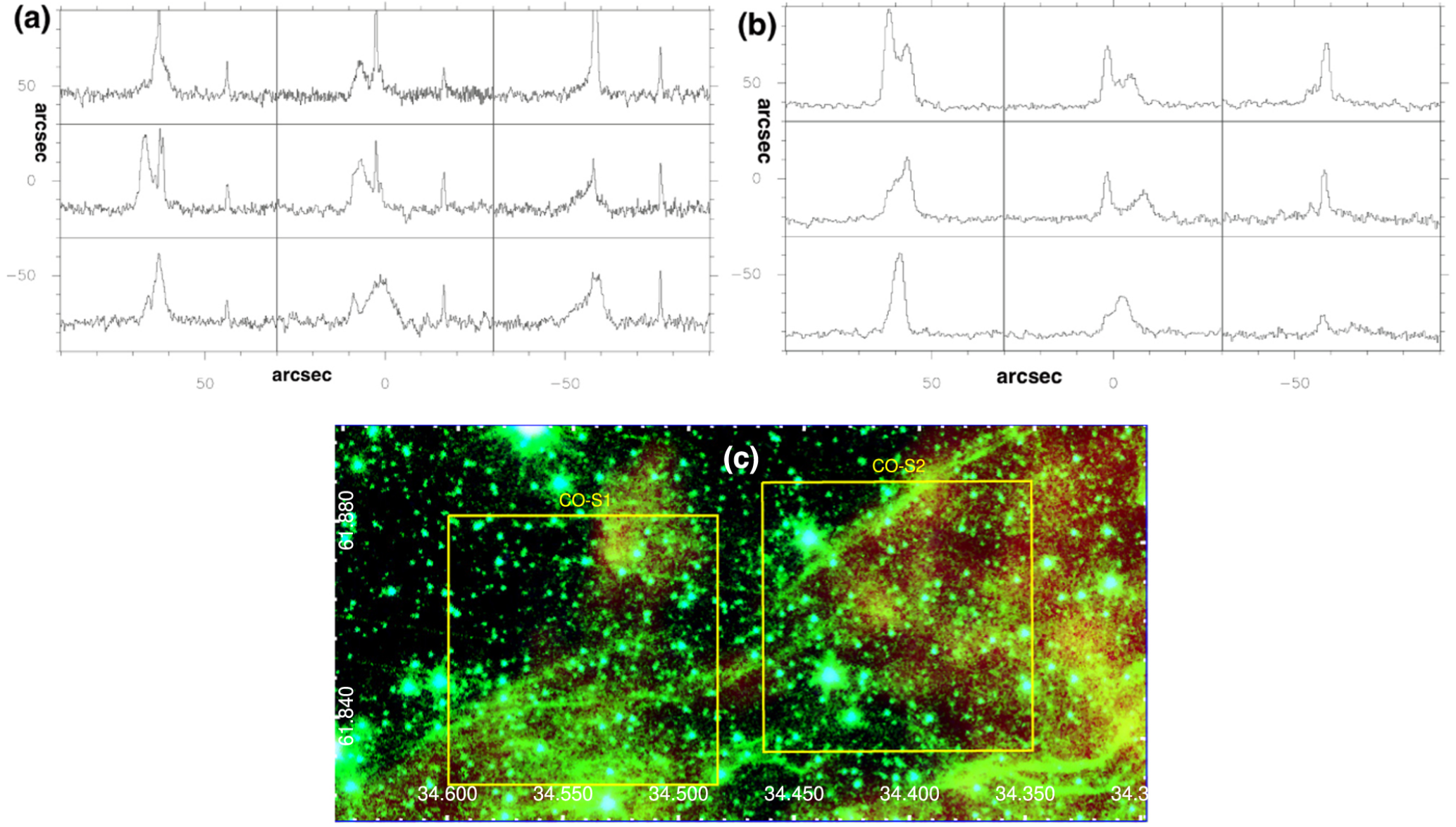
Figure 9. from Shocked Molecular Hydrogen and Broad CO Lines from the Interacting Supernova Remnant HB 3 null 2021 APJ 917 47 doi:10.3847/1538-4357/ac08a4 https://dx.doi.org/10.3847/1538-4357/ac08a4 © 2021. The American Astronomical Society. All rights reserved.
