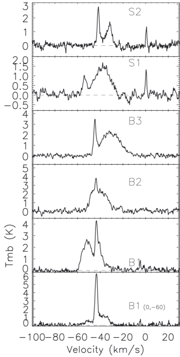
Figure 8. from Shocked Molecular Hydrogen and Broad CO Lines from the Interacting Supernova Remnant HB 3 null 2021 APJ 917 47 doi:10.3847/1538-4357/ac08a4 https://dx.doi.org/10.3847/1538-4357/ac08a4 © 2021. The American Astronomical Society. All rights reserved.
