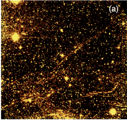
Figure 6. from Shocked Molecular Hydrogen and Broad CO Lines from the Interacting Supernova Remnant HB 3 null 2021 APJ 917 47 doi:10.3847/1538-4357/ac08a4 https://dx.doi.org/10.3847/1538-4357/ac08a4 © 2021. The American Astronomical Society. All rights reserved.
