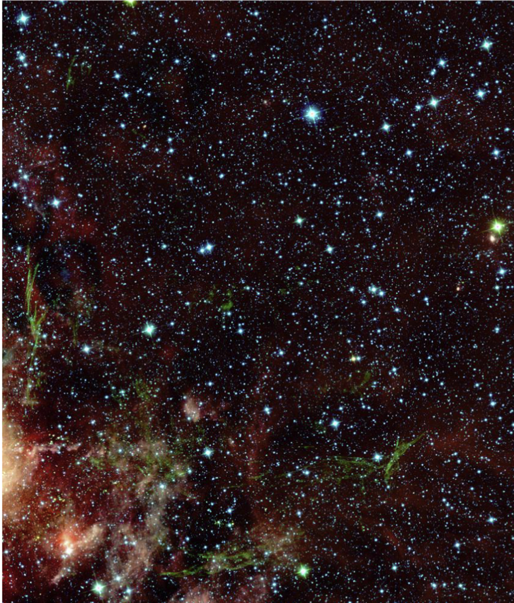
Figure 3. from Shocked Molecular Hydrogen and Broad CO Lines from the Interacting Supernova Remnant HB 3 null 2021 APJ 917 47 doi:10.3847/1538-4357/ac08a4 https://dx.doi.org/10.3847/1538-4357/ac08a4 © 2021. The American Astronomical Society. All rights reserved.
