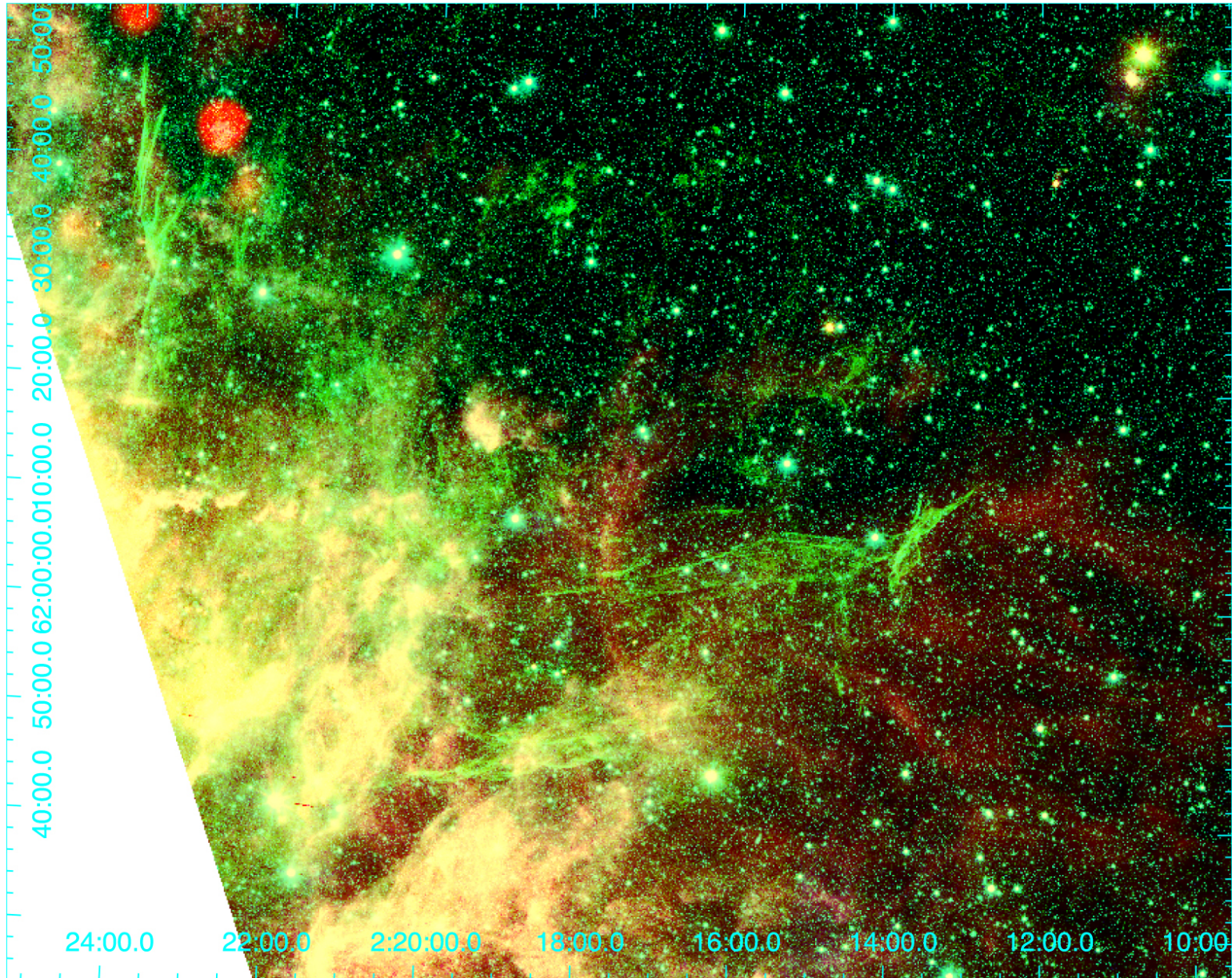
Figure 2. from Shocked Molecular Hydrogen and Broad CO Lines from the Interacting Supernova Remnant HB 3 null 2021 APJ 917 47 doi:10.3847/1538-4357/ac08a4 https://dx.doi.org/10.3847/1538-4357/ac08a4 © 2021. The American Astronomical Society. All rights reserved.
