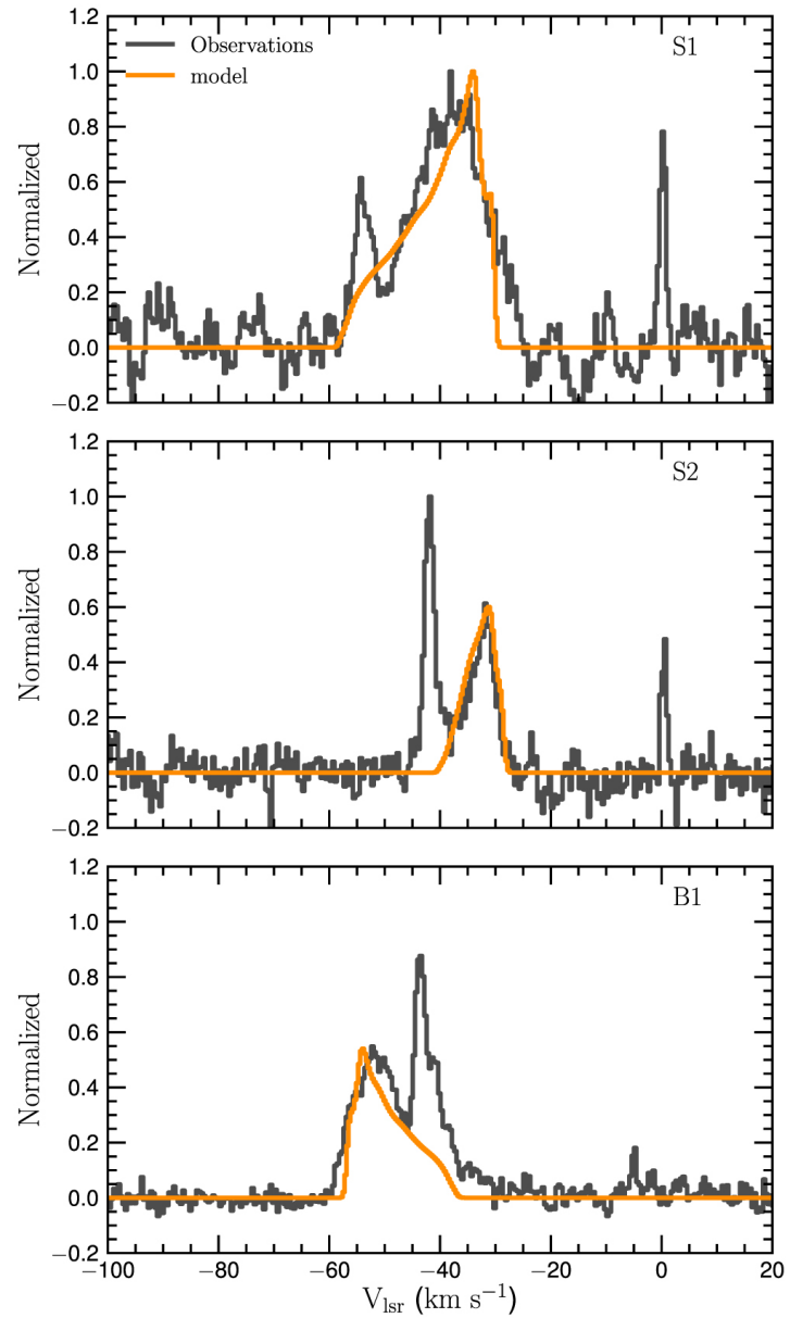
Figure 16. from Shocked Molecular Hydrogen and Broad CO Lines from the Interacting Supernova Remnant HB 3 null 2021 APJ 917 47 doi:10.3847/1538-4357/ac08a4 https://dx.doi.org/10.3847/1538-4357/ac08a4
