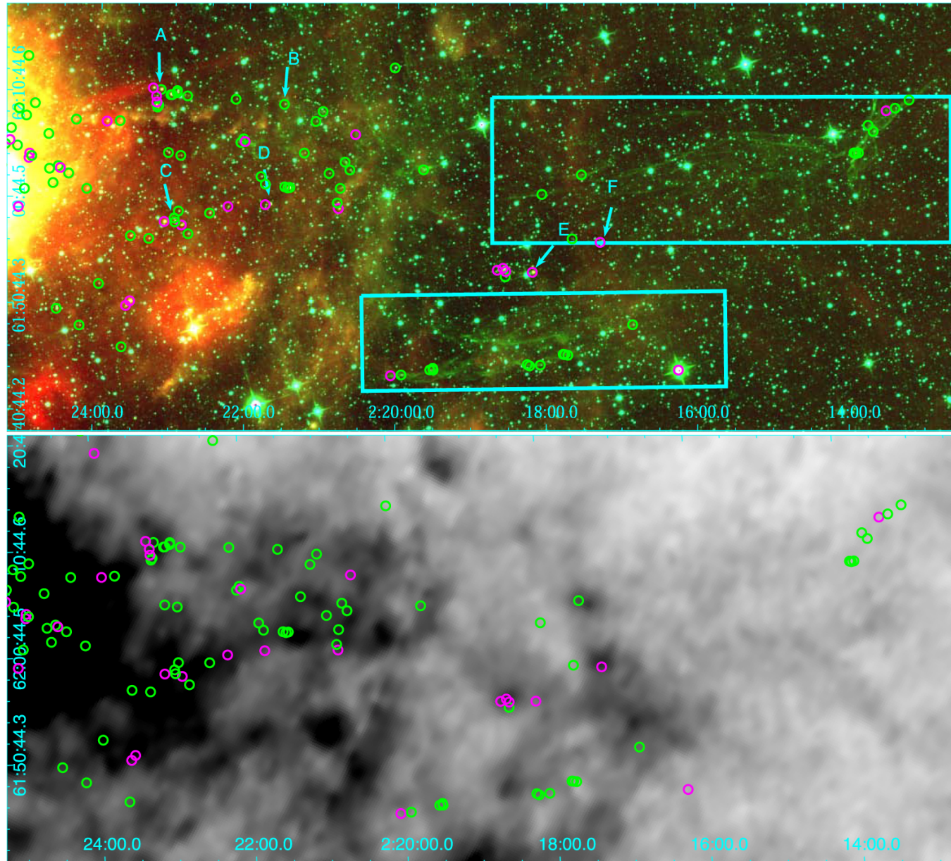
Figure 15. from Shocked Molecular Hydrogen and Broad CO Lines from the Interacting Supernova Remnant HB 3 null 2021 APJ 917 47 doi:10.3847/1538-4357/ac08a4 https://dx.doi.org/10.3847/1538-4357/ac08a4 © 2021. The American Astronomical Society. All rights reserved.
