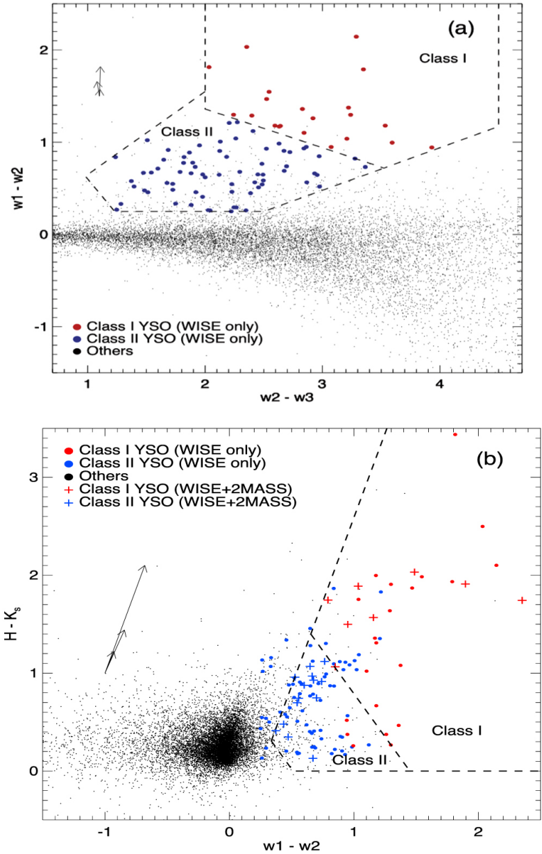
Figure 14. from Shocked Molecular Hydrogen and Broad CO Lines from the Interacting Supernova Remnant HB 3 null 2021 APJ 917 47 doi:10.3847/1538-4357/ac08a4 https://dx.doi.org/10.3847/1538-4357/ac08a4 © 2021. The American Astronomical Society. All rights reserved.
