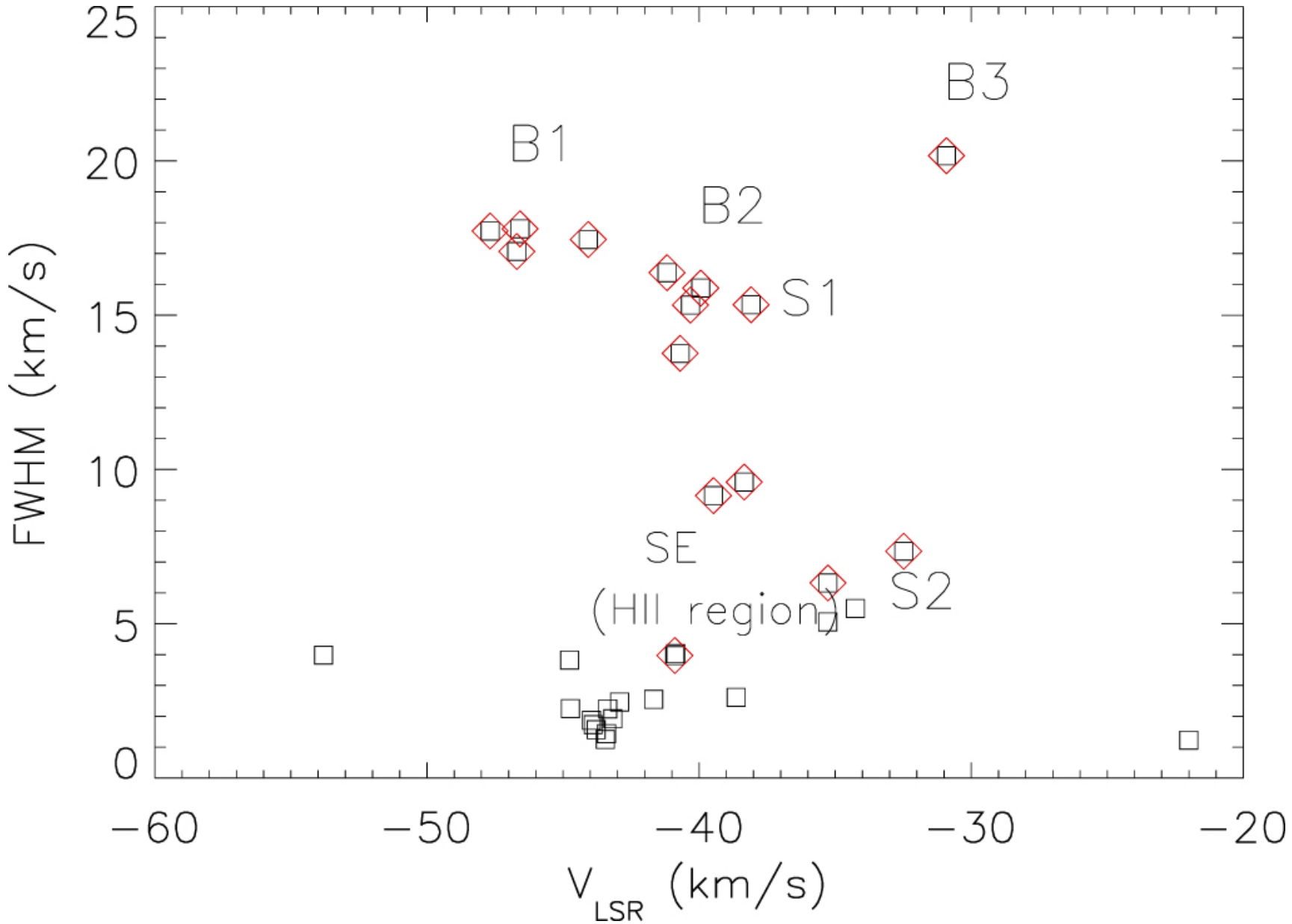
Figure 12. from Shocked Molecular Hydrogen and Broad CO Lines from the Interacting Supernova Remnant HB 3 null 2021 APJ 917 47 doi:10.3847/1538-4357/ac08a4 https://dx.doi.org/10.3847/1538-4357/ac08a4 © 2021. The American Astronomical Society. All rights reserved.
