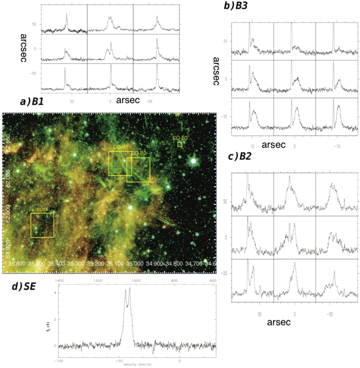
Figure 10. from Shocked Molecular Hydrogen and Broad CO Lines from the Interacting Supernova Remnant HB 3 null 2021 APJ 917 47 doi:10.3847/1538-4357/ac08a4 https://dx.doi.org/10.3847/1538-4357/ac08a4 © 2021. The American Astronomical Society. All rights reserved.
