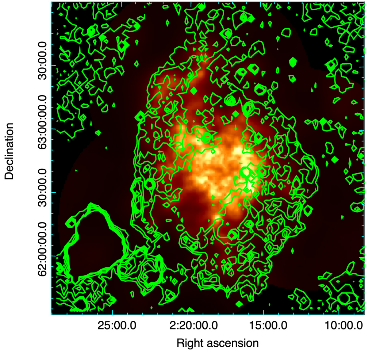
Figure 1. from Shocked Molecular Hydrogen and Broad CO Lines from the Interacting Supernova Remnant HB 3 null 2021 APJ 917 47 doi:10.3847/1538-4357/ac08a4 https://dx.doi.org/10.3847/1538-4357/ac08a4 © 2021. The American Astronomical Society. All rights reserved.
