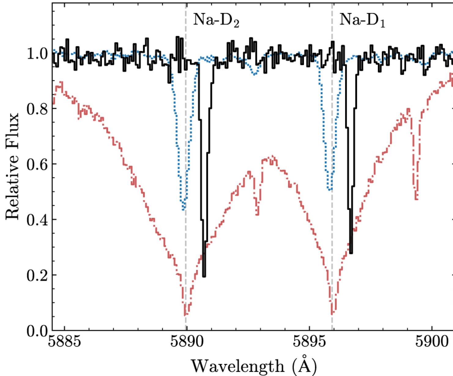
Figure 8. from Recurring Planetary Debris Transits and Circumstellar Gas around White Dwarf ZTF J0328–1219 null 2021 APJ 917 41 doi:10.3847/1538-4357/ac0822 https://dx.doi.org/10.3847/1538-4357/ac0822 © 2021. The American Astronomical Society. All rights reserved.
