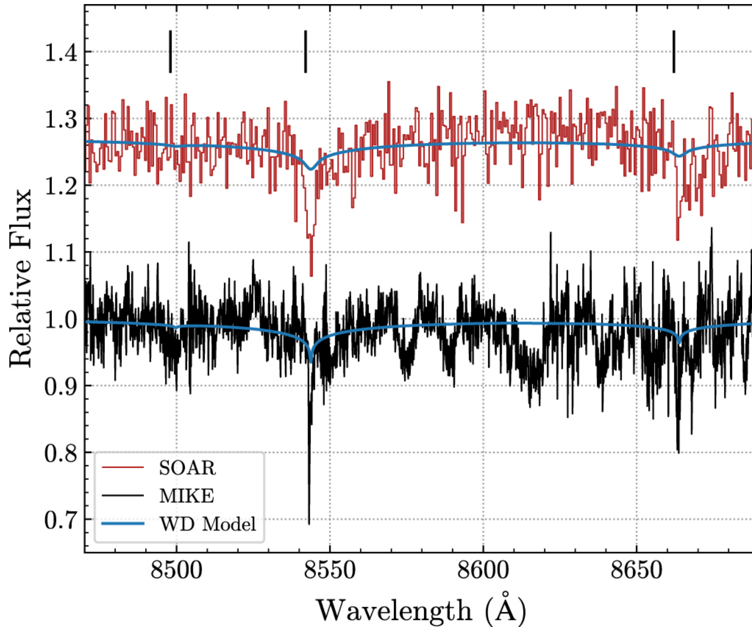
Figure 7. from Recurring Planetary Debris Transits and Circumstellar Gas around White Dwarf ZTF J0328–1219 null 2021 APJ 917 41 doi:10.3847/1538-4357/ac0822 https://dx.doi.org/10.3847/1538-4357/ac0822 © 2021. The American Astronomical Society. All rights reserved.
