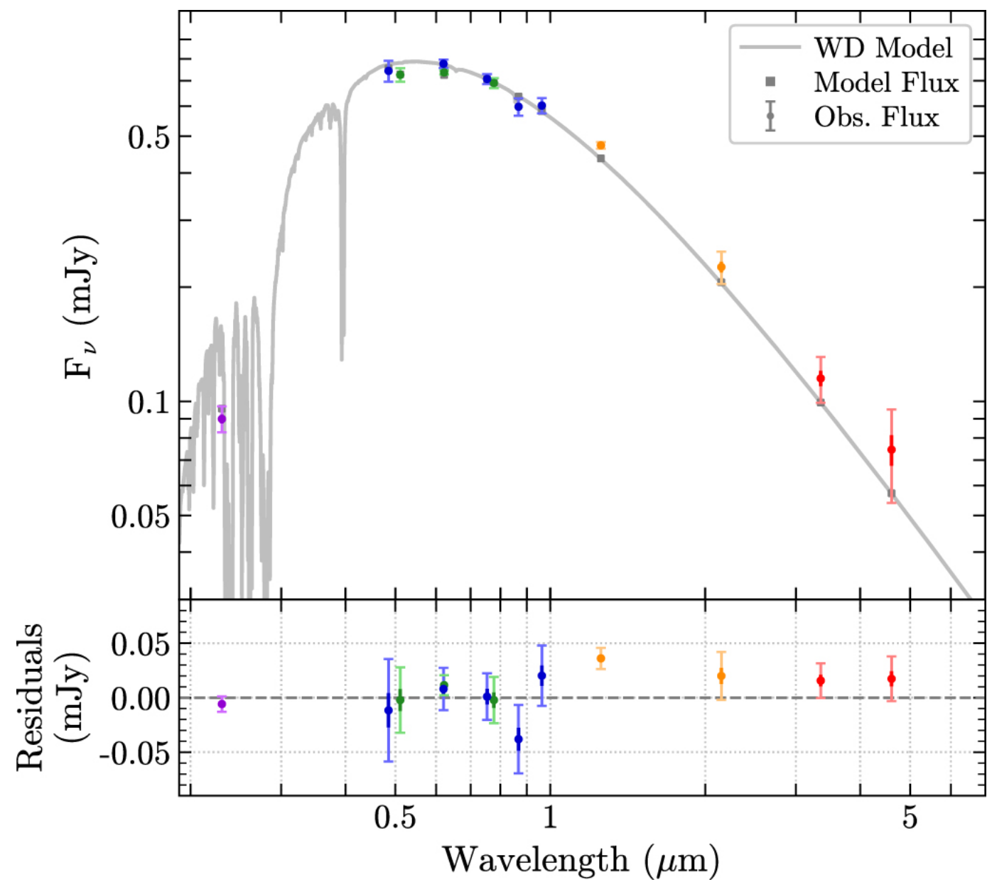
Figure 6. from Recurring Planetary Debris Transits and Circumstellar Gas around White Dwarf ZTF J0328–1219 null 2021 APJ 917 41 doi:10.3847/1538-4357/ac0822 https://dx.doi.org/10.3847/1538-4357/ac0822 © 2021. The American Astronomical Society. All rights reserved.
