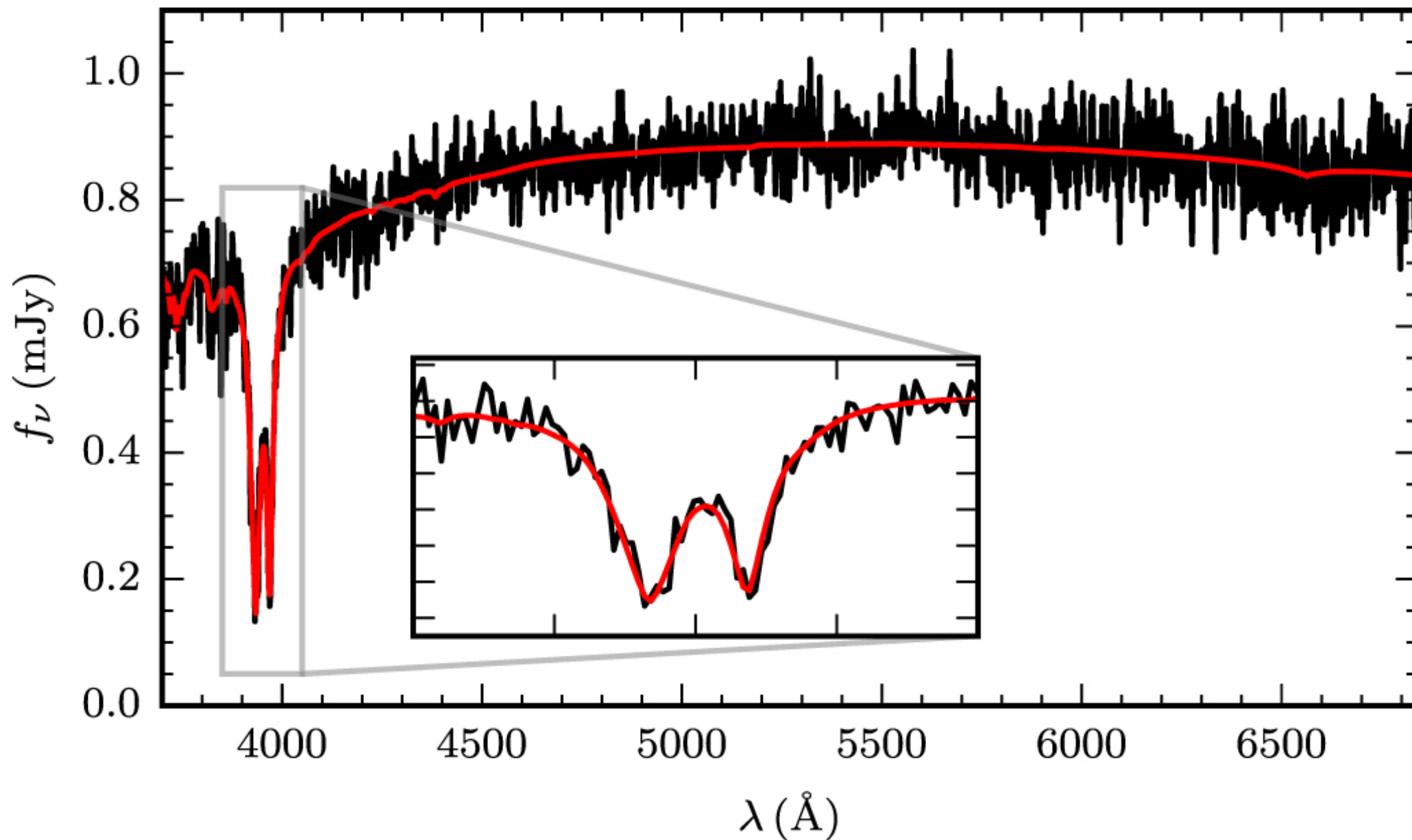
Figure 5. from Recurring Planetary Debris Transits and Circumstellar Gas around White Dwarf ZTF J0328–1219 null 2021 APJ 917 41 doi:10.3847/1538-4357/ac0822 https://dx.doi.org/10.3847/1538-4357/ac0822 © 2021. The American Astronomical Society. All rights reserved.
